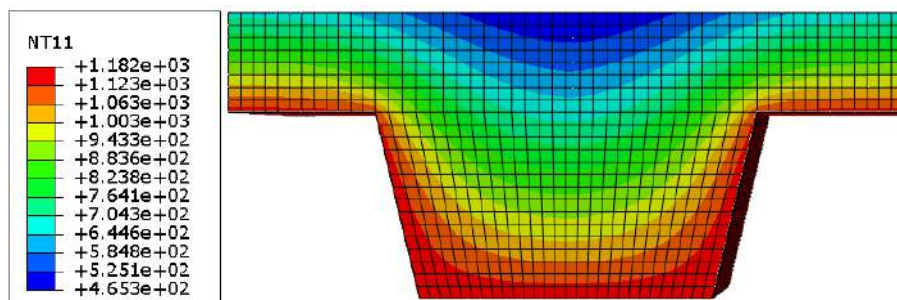
Figura 217 – Isotermas h_c=40\text{mm} ( h_f = 75\text{mm} )
