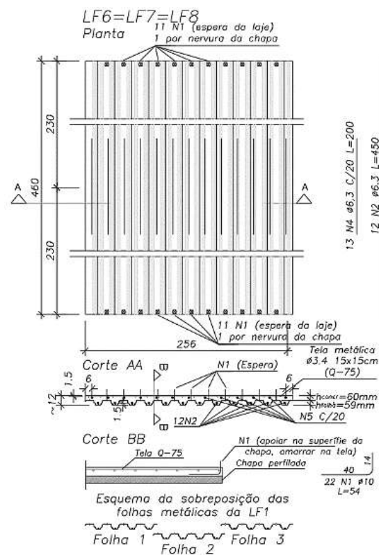
(l) LF6, LF7 e LF8
