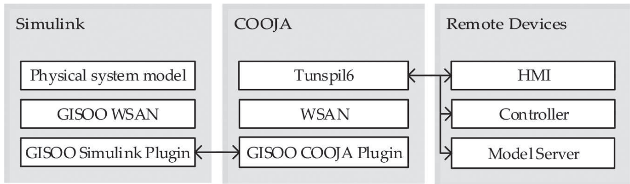
Figure 6. Testbed simulator.
