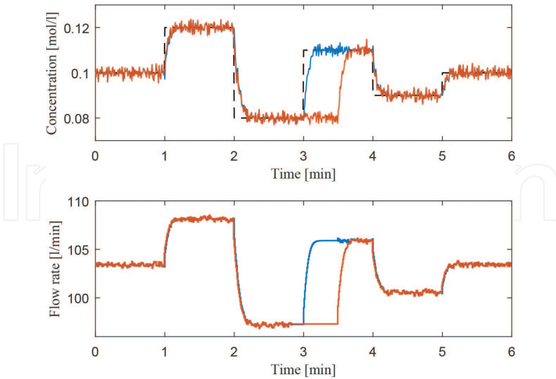
Figure 12. CSTR system: node lost.
