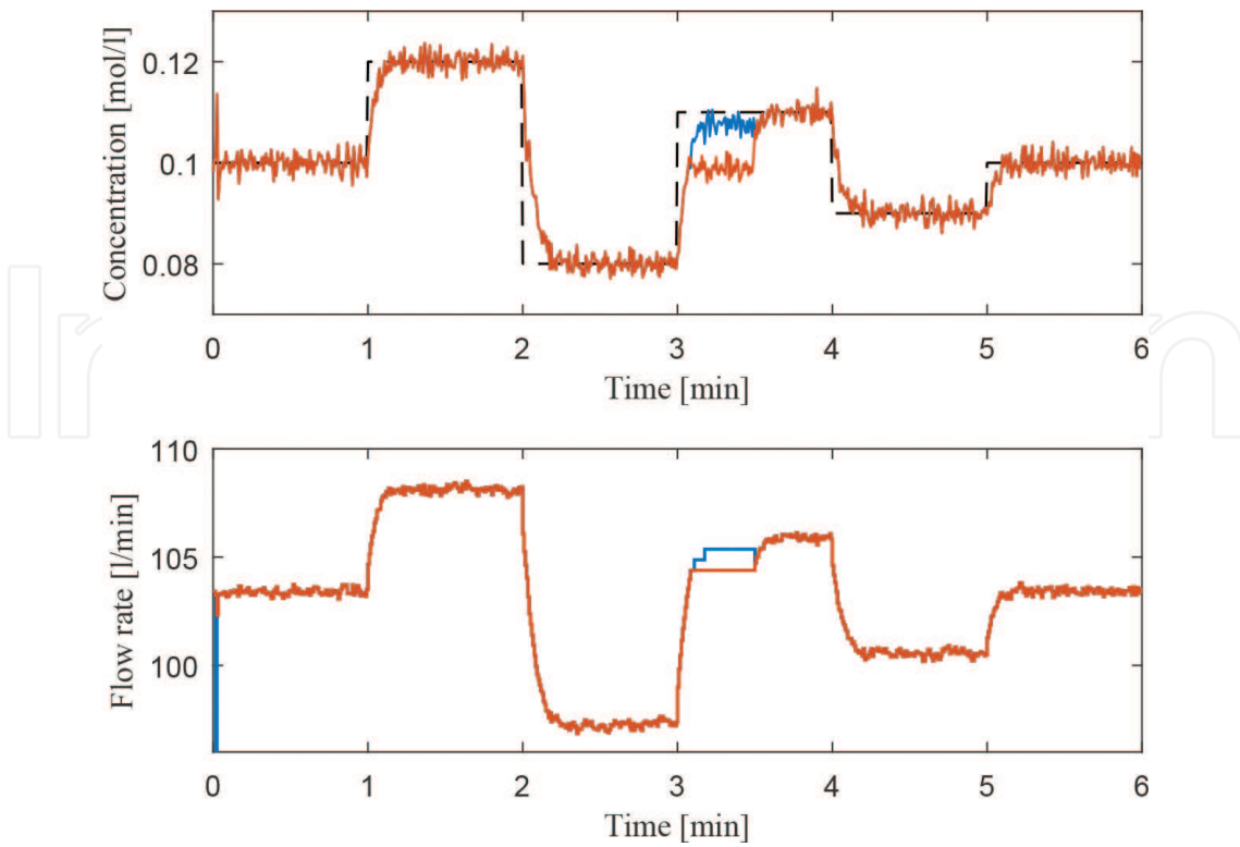
Figure 11. CSTR system: jamming attack.
