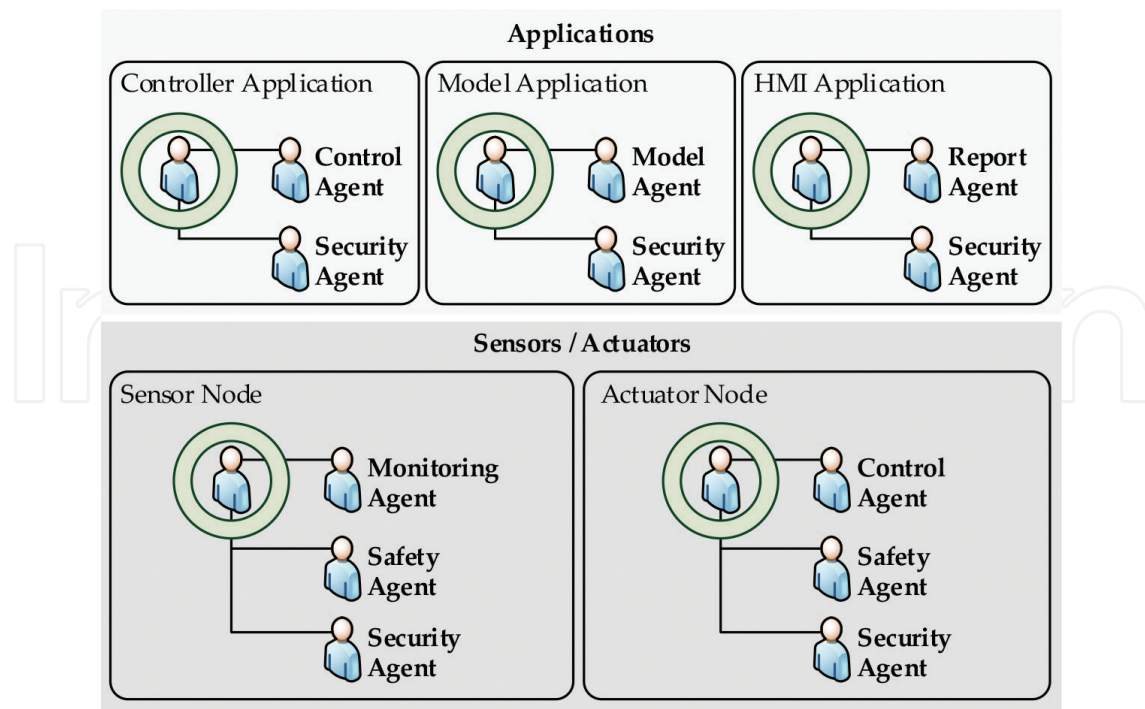
Figure 10. Multiagent framework.
