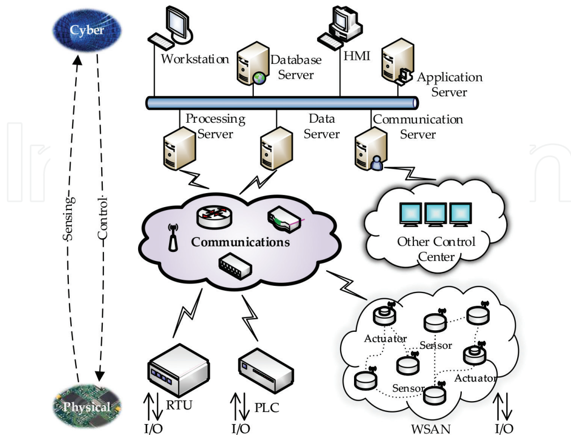
Figure 1. Example of a cyber-physical system.
