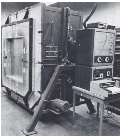
Figure 2.38 – High-temperature guarded hot box: a) vertical cross-section; b) facility photography [161].
