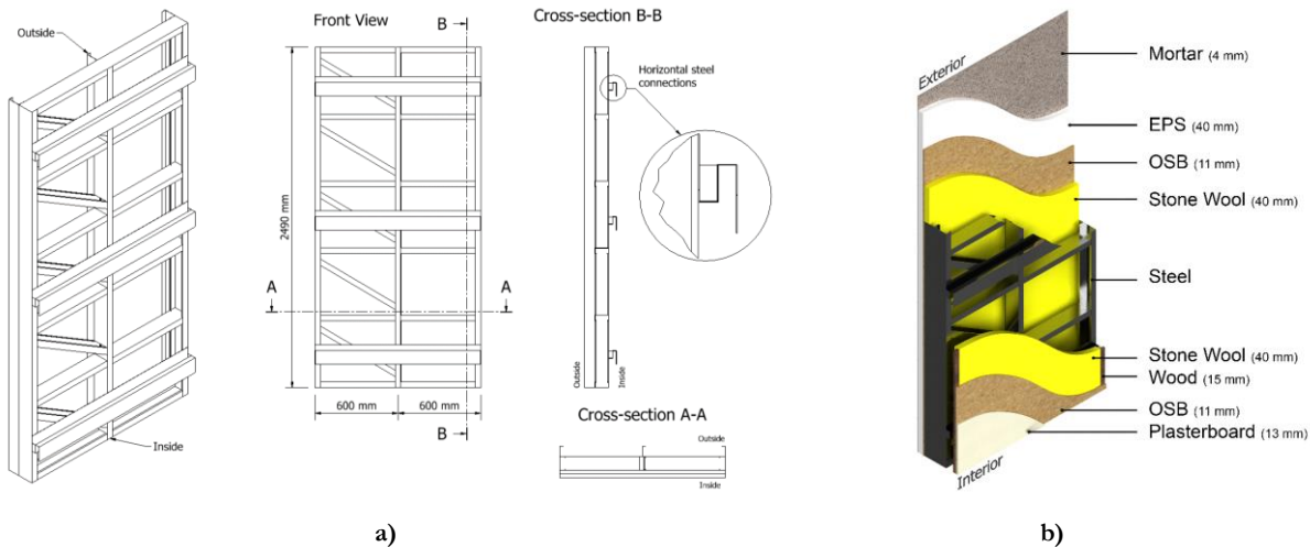
Figure 5.11 – LSF wall model used in the previous parametric study: a) steel structure; and b) wall module materials [50].
