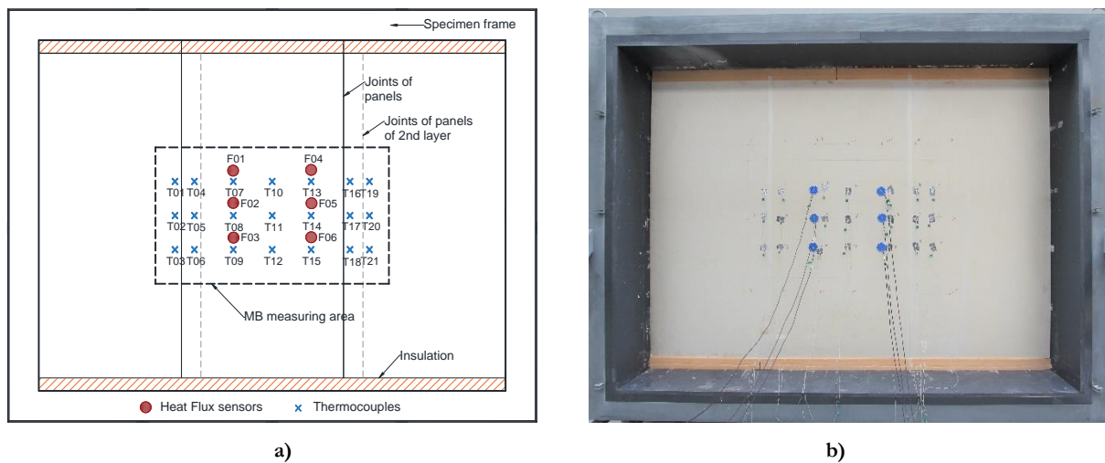
Figure 4.68 – Location of temperature and heat flux sensors placed on the GHB cold side of the calcium silicate boards wall surface: a) sketch; b) photo.
