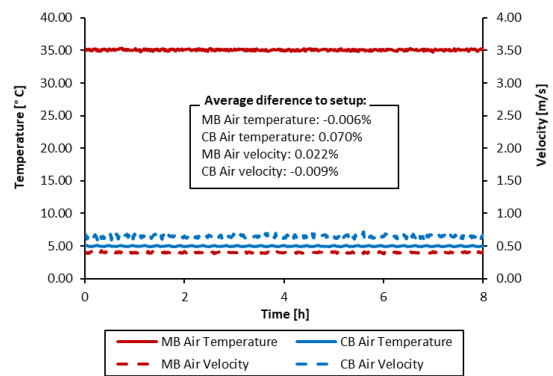
Figure 4.74 – Test M03.C019 air temperature and velocity in chambers for GHB with calcium silicate boards.
