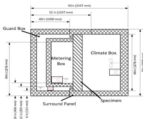
Figure 2.81 – GHB schematics cross section [220].
