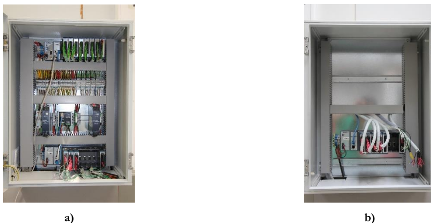
Figure 4.17 – Control and data logging panels: a) main with CompactRIO Controller model cRIO-9074 on the top and the expansion unit NI 9144 8-slot in the bottom; b) secondary with the other expansion unit NI 9144 8-slot.
