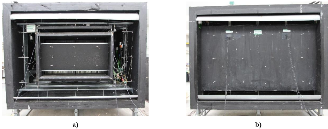
Figure 4.10 – Sensors a) GHB metering box; b) cold box.
