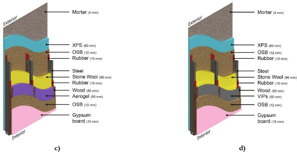
Figure 5.19 – Models with the combined improvement strategies: a) Model H; b) Model I; c) Model J; and d) Model K.
