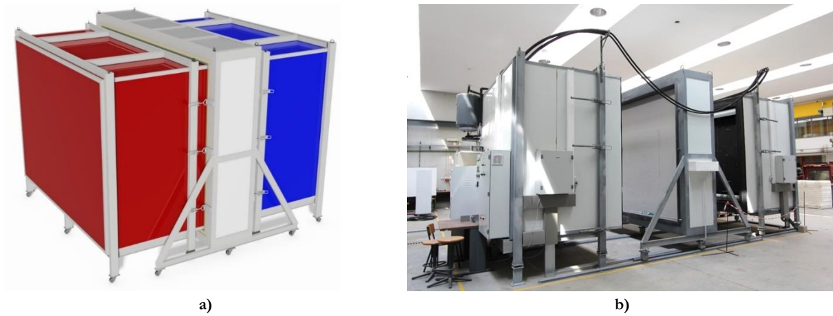
Figure 4.1 – Hot box apparatus: a) sketch from the design phase of the equipment closed; b) photography of the equipment open.
