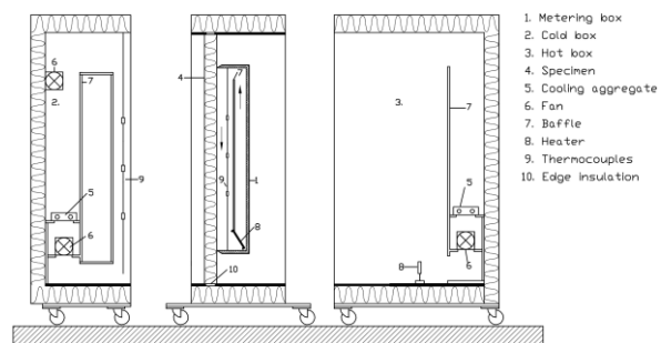
Figure 2.68 – GHB vertical cross-section [197].
