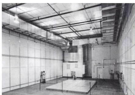
Figure 2.45 – Calibrated hot box apparatus interior of Thermal Research Facility [166].
