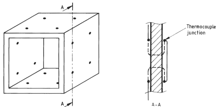
Figure 3.6 – Thermocouple connections to form metering box thermopile [277].
