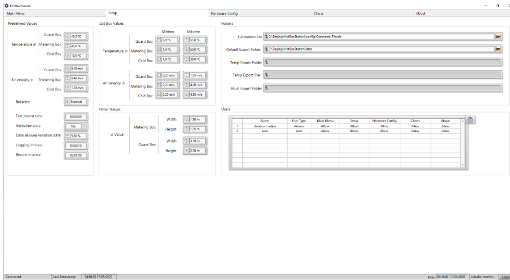
Figure 4.19 – Software Setup.
