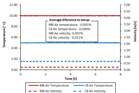
Figure 4.81 – Test M03.C156 air temperature and velocity in chambers for CHB with EPS panels 50 mm thick.
