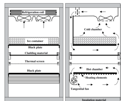
Figure 2.72 – Hot box [204].
