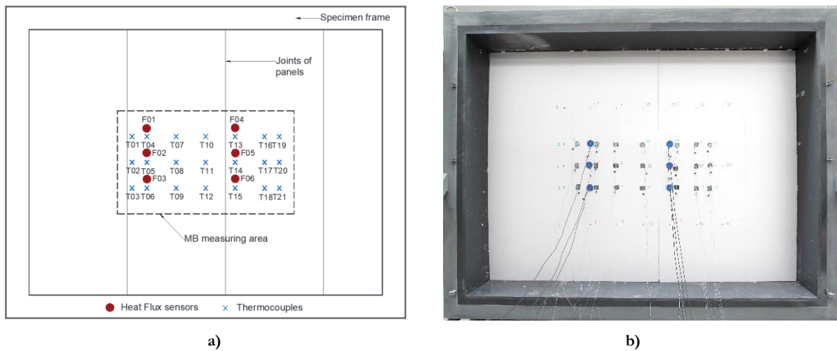
Figure 4.82 – Location of temperature and heat flux sensors placed on the GHB cold side of the EPS 50 mm thick wall surface: a) sketch; b) photo.
