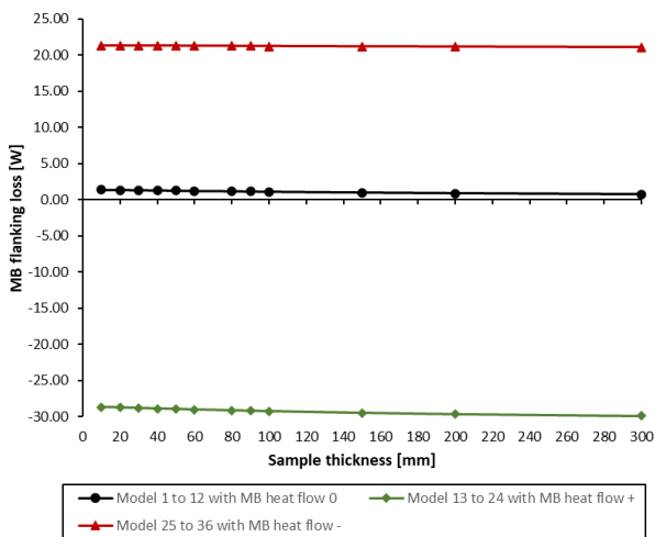
Figure 4.29 – Relationship of MB walls flanking loss to specimen thickness, for models 1 to 36, for CHB of a specimen with specimen \lambda=0.036 \text{ W}/(\text{m.K}) .
