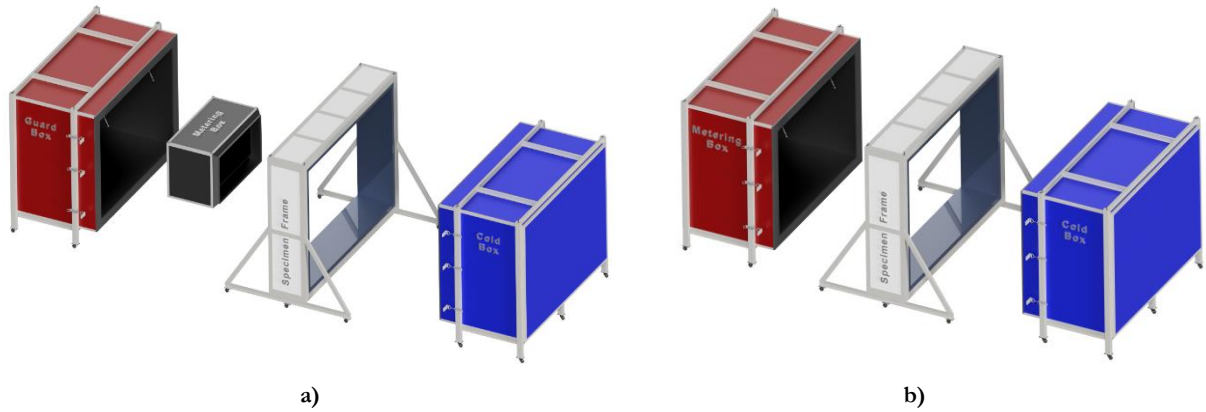
Figure 4.2 – Apparatus passive components: a) GHB; b) CHB.
