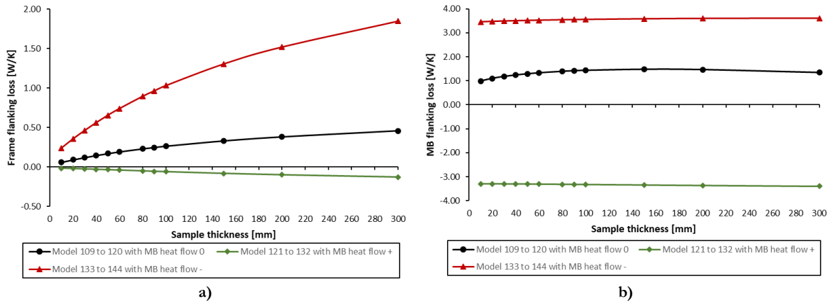
Figure 4.34 – Relationship of flanking loss to specimen thickness, estimated with modelling, for models 109 to 144 for CHB of a specimen with specimen \lambda=0.175 W/(m.K) of: a) Specimen frame; and b) MB walls.
