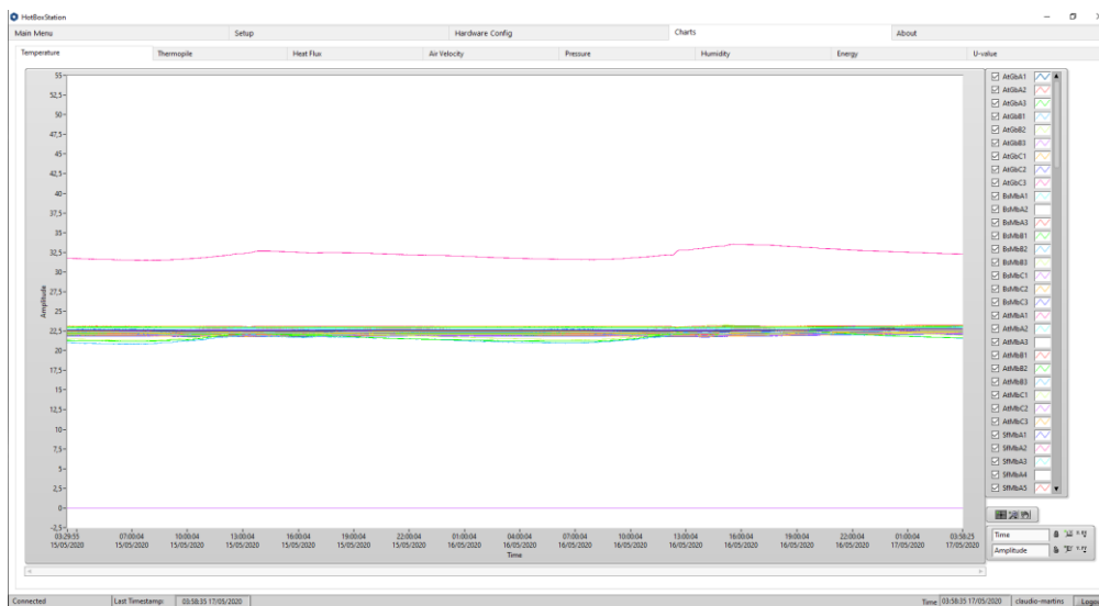
Figure 4.21 – Software Charts.
