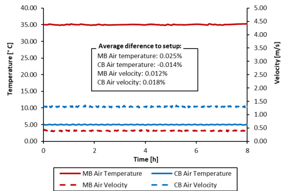
Figure 4.102 – Test M12.C255 air temperature and velocity in chambers of test cases with MB wall heat flux negative for GHB with EPS panels 100 mm thick.
