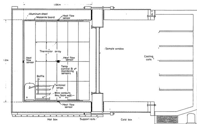
Figure 2.39 – Calibrated hot box vertical section [162].
