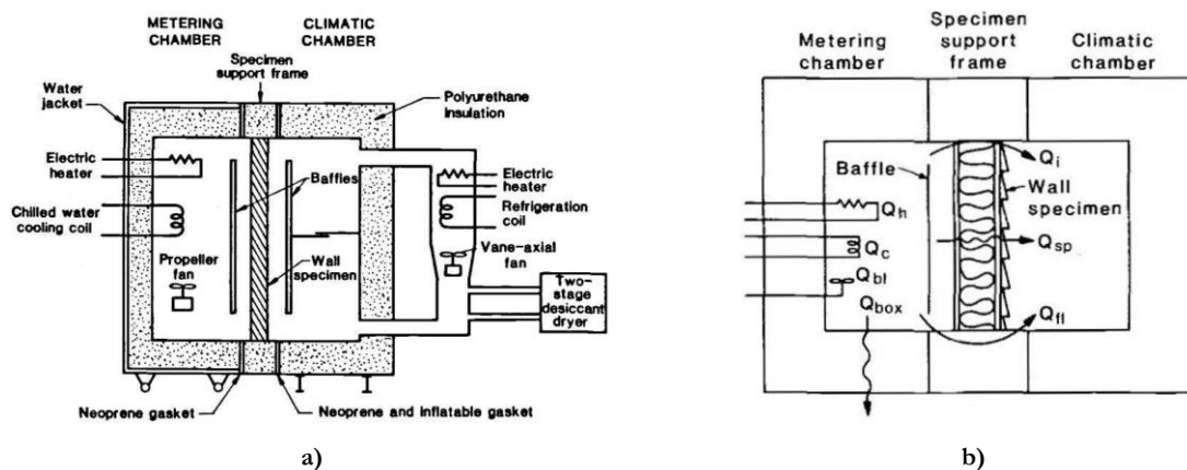
Figure 2.55 – CHB facility of the National Institute of Standards and Technology: a) schematic cross-section; b) energy balance of metering chamber under dynamic conditions [89].
