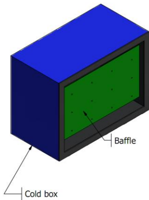
Figure A.10 – Air temperature sensors in cold box, between specimen and baffle.
