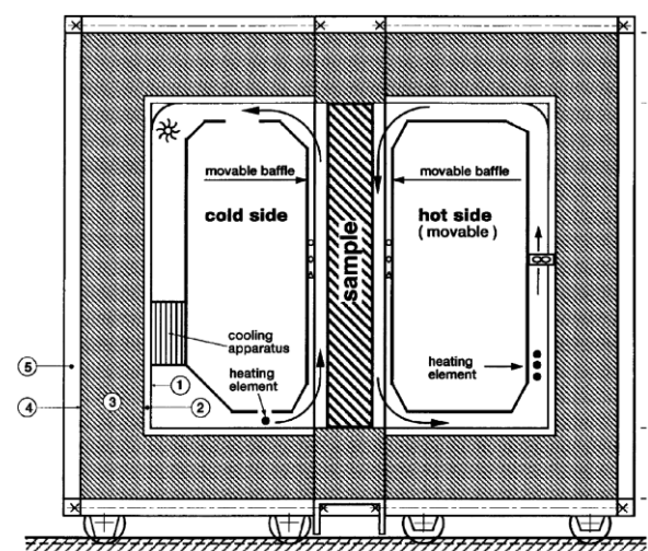
Figure 2.65 – Schematic cross-section of the CHB [194].
