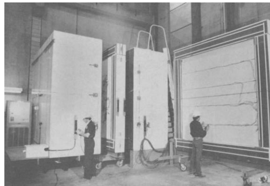
Figure 2.52 – CHB facility of Construction Technology Laboratories, Portland Cement Association [177].
