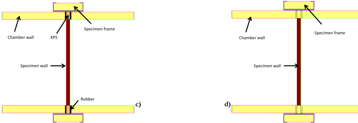
Figure 4.24 – Numerical models of the specimen placed directly: c) surrounded of insulation with 200 mm; d) reference model.
