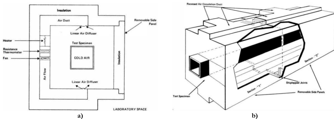
Figure 2.37 – Calibrated hot box apparatus schematic: a) vertical cross-section; b) with the installed specimen [160].
