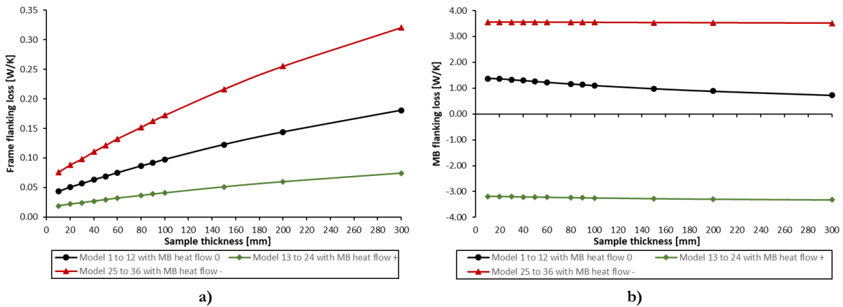
Figure 4.28 – Relationship of flanking loss to specimen thickness, estimated with modelling, for models 1 to 36, for CHB of a specimen with specimen \lambda=0.036 \text{ W}/(\text{m.K}) of: a) Specimen frame; and b) MB walls.
