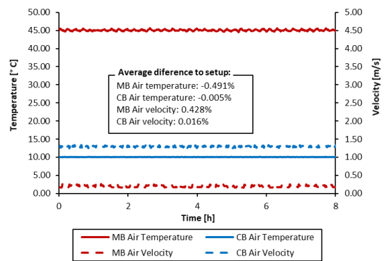
Figure 4.88 – Test M15.C192 air temperature and velocity in chambers for GHB with EPS panels 50 mm thick.
