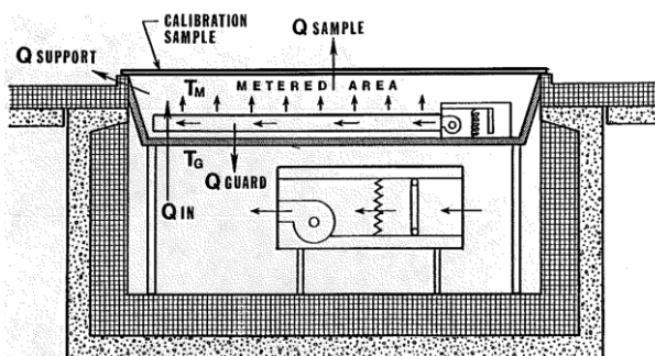
Figure 2.40 – Large-scale horizontal calibrated hot box: a) metering chamber schematic; b) room facility shown the calibration sample installed over the metering chamber [163].
