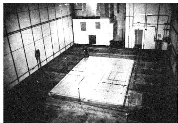
Figure 2.40 – Large-scale horizontal calibrated hot box: a) metering chamber schematic; b) room facility shown the calibration sample installed over the metering chamber [163].
