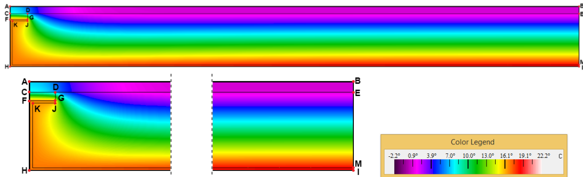
Figure 2.16 – Test case number 2 in THERM.
