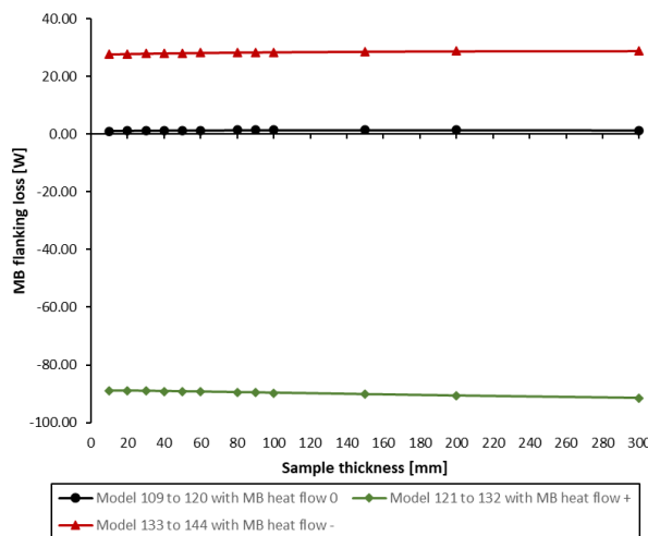
Figure 4.35 – Relationship of MB walls flanking loss to specimen thickness, for models 109 to 144, for CHB of a specimen with specimen \lambda=0.175 W/(m.K).
