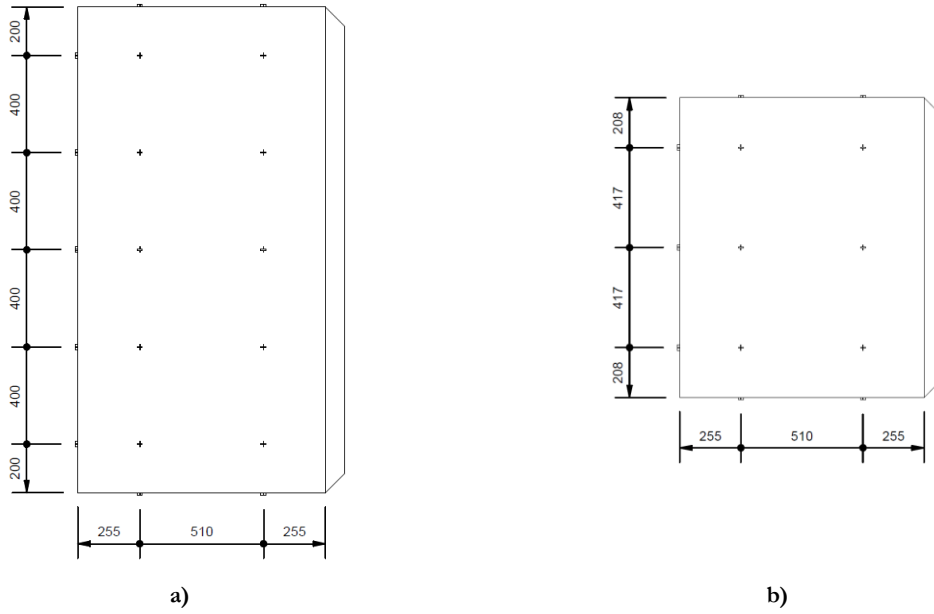
Figure B.2 – Thermopile of GHB metering box: a) Top view; b) Front view.
