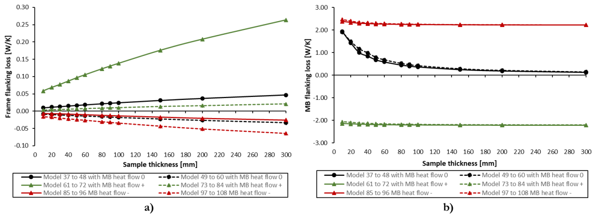
Figure 4.30 – Relationship of flanking loss to specimen thickness, estimated with modelling, for models 37 to 108, for GHB of a specimen with specimen \lambda=0.036 \text{ W}/(\text{m.K}) of: a) Specimen frame; and b) MB walls.
