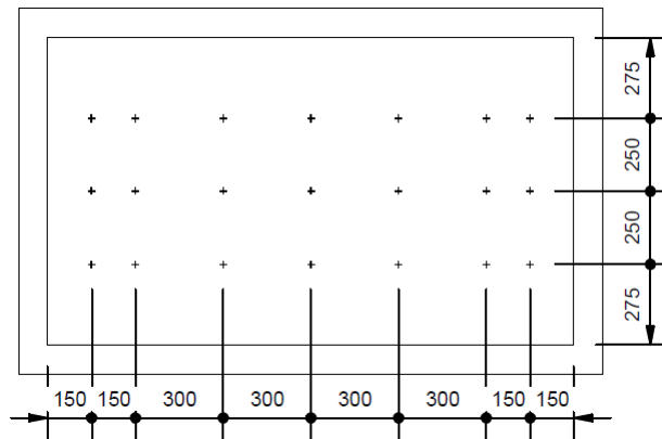
Figure A.2 – Specimen surface temperature sensors inside the metering and cold box – front view.
