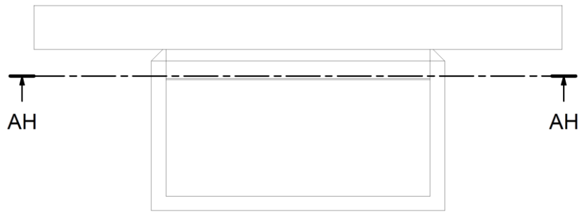
Figure C.4 – Air velocity sensors of metering box (GHB) top view.
