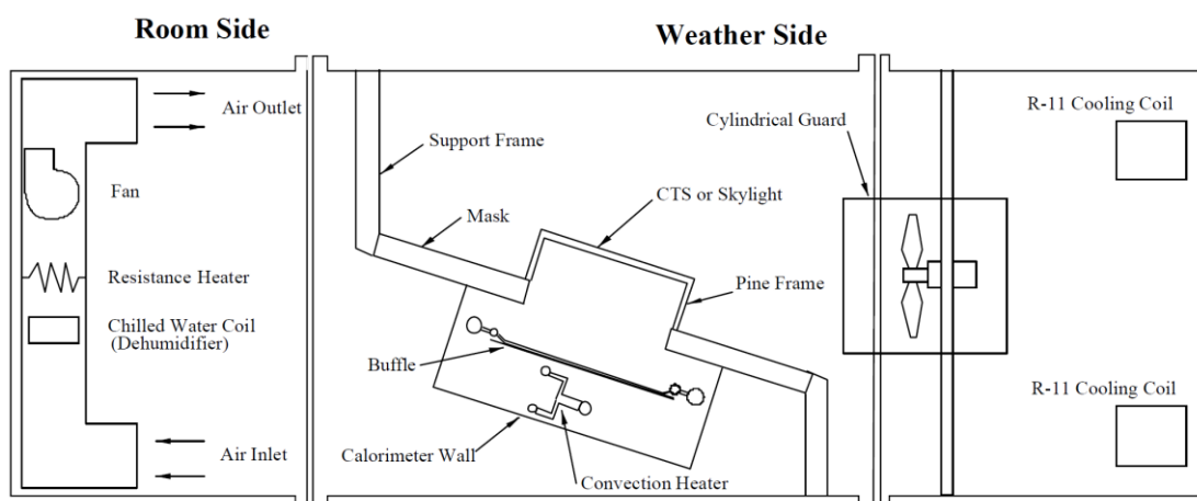
Figure 2.61 – Schematic of the hot box facility for inclined skylight testing [188].
