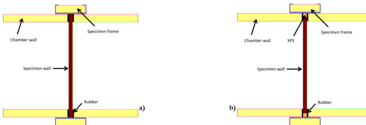
Figure 4.24 – Numerical models of the specimen placed directly: a) on the specimen frame; b) surrounded of insulation with 100 mm.
