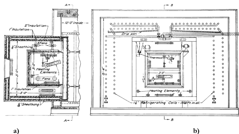
Figure 2.24 – Hot box: a) sectional view of the double box and wall in place; b) sectional view of the cold room, by looking into the open end of test room [146].
