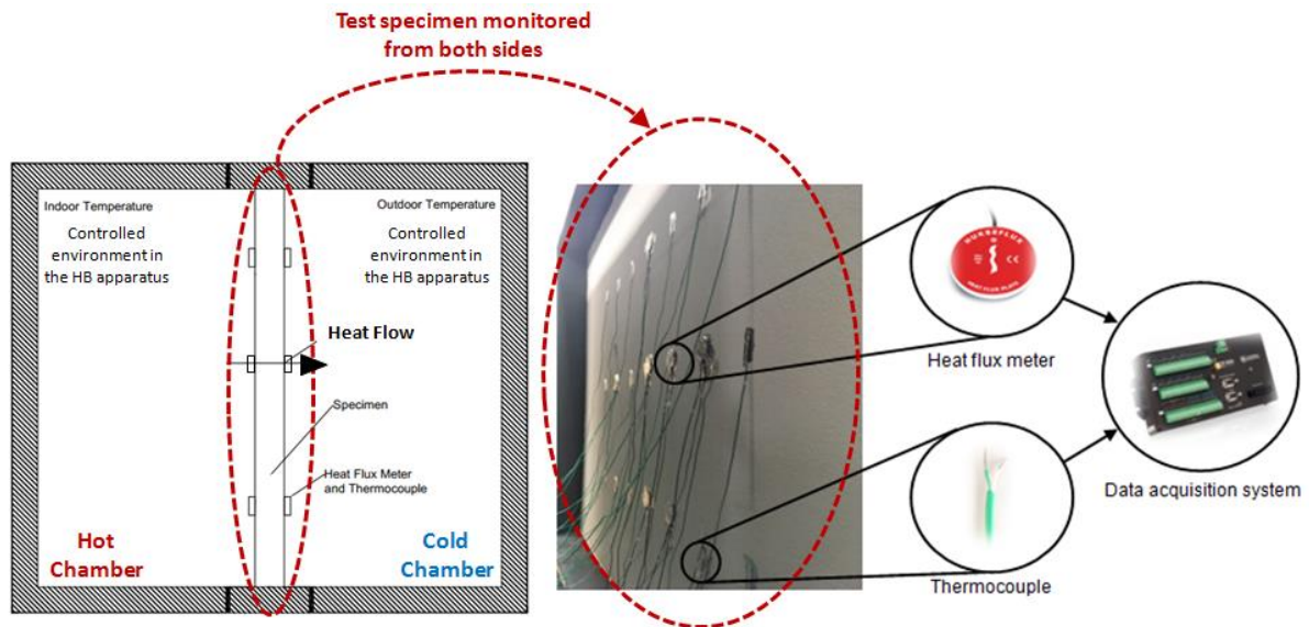
Figure 2.9 – The instrumented outer surface of an LSF wall (test sample): a sketch of the application of the HFM method in a laboratory-controlled environment [59].
