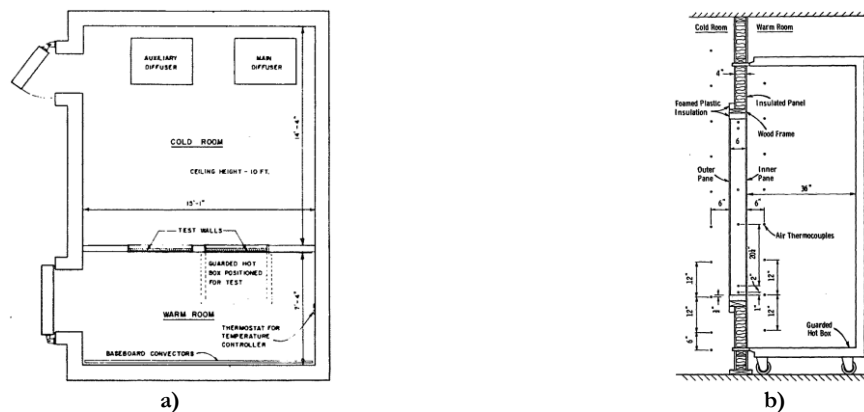
Figure 2.28 – Guard hot box: a) plant view of the equipment [80]; b) schematic cross section [151].
