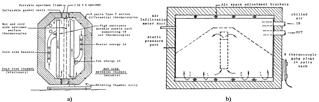
Figure 2.44 – Calibrated hot box apparatus: a) side cross-section; b) cold side frontal cross section [165].
