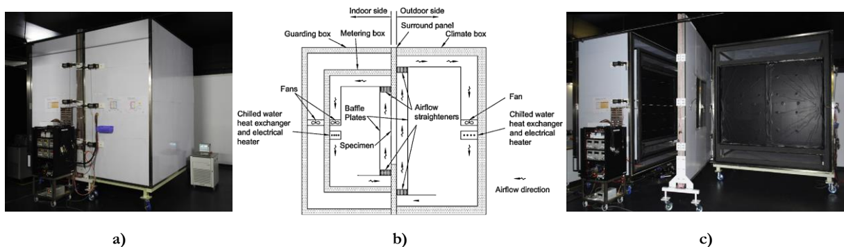
Figure 2.77 – GHB: a) side view; b) schematics vertical cross section; c) side view with the apparatus open [1].
