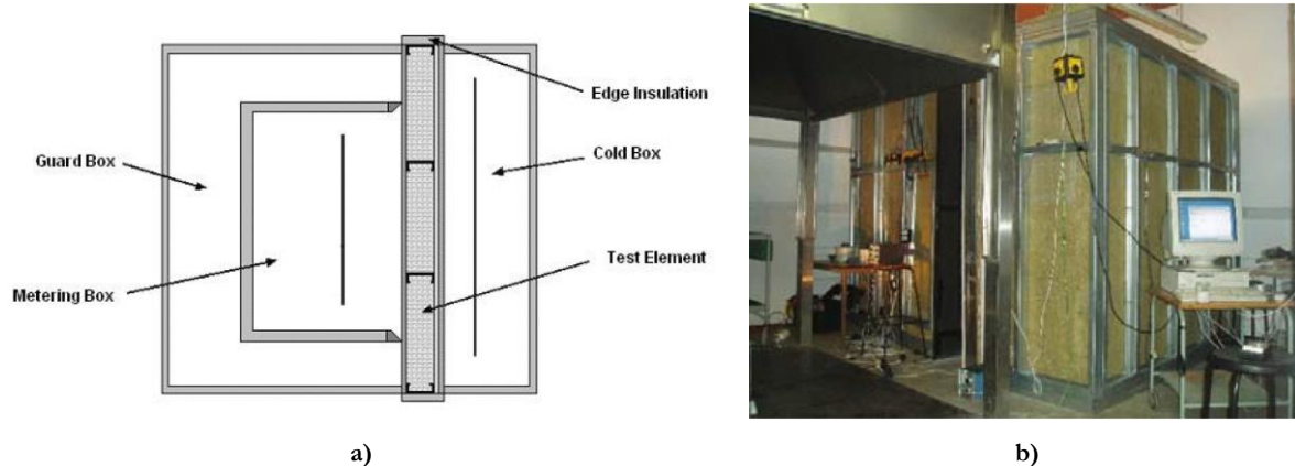
Figure 2.80 –GHB: a) schematic; b) apparatus [218].
