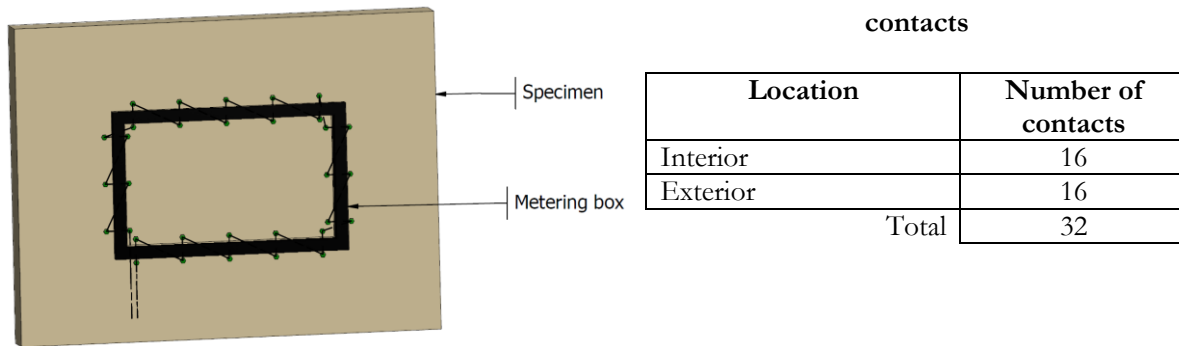
Figure B.4 – Thermopile of GHB metering box perimeter seal.
