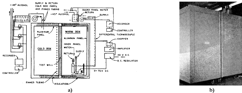
Figure 2.27 – Calibrated hot box: a) Cross-section sketch view; b) Photography of the equipment [86].
