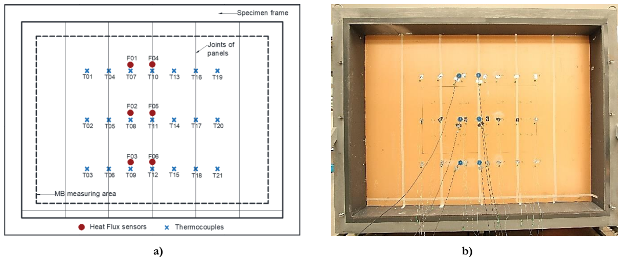
Figure 4.46 – Location of temperature and heat flux sensors placed on the CHB cold side of the XPS wall surface: a) sketch; b) photo.
