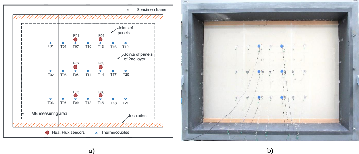
Figure 4.61 – Location of temperature and heat flux sensors placed on the CHB cold side of the calcium silicate boards wall surface: a) sketch; b) photo.
