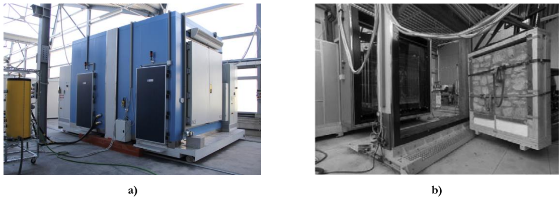
Figure 2.86 – Guarded hot box test: a) apparatus [229]; b) specimen [230].
