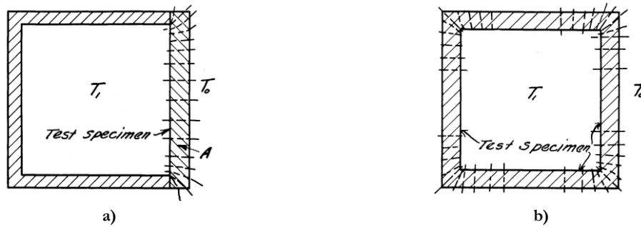
Figure 2.21 – Hot Box method: a) testing over one open side; b) testing a complete cubical of the material [28].
