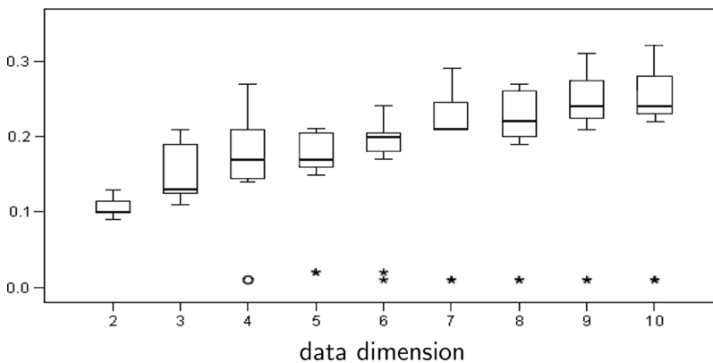
Figure 5. Empirical distribution of h_{f,n} for several values of d at level 0.05.
