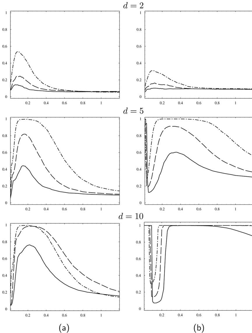
Figure 4. Empirical power of I_n^2(h) as function of h for n = 10 (solid line), n = 20 (broken line), n = 40 (broken and dotted line), and d = 2, 5, 10 at level 0.05: (a) AL_d(0, \Sigma_{0.2}) ; (b) K_d(1, 0, \Sigma_{0.5}) .
