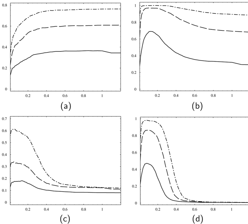
Figure 3. Empirical power of I_n^2(h) as function of h for n = 20 (solid line), n = 40 (broken line), and n = 60 (broken and dotted line) at level 0.05: (a) Beta(0.75,1.125); (b) Beta(1.5,2.25); (c) Beta(0.5,0.5); (d) Beta(2.5,2.5).
