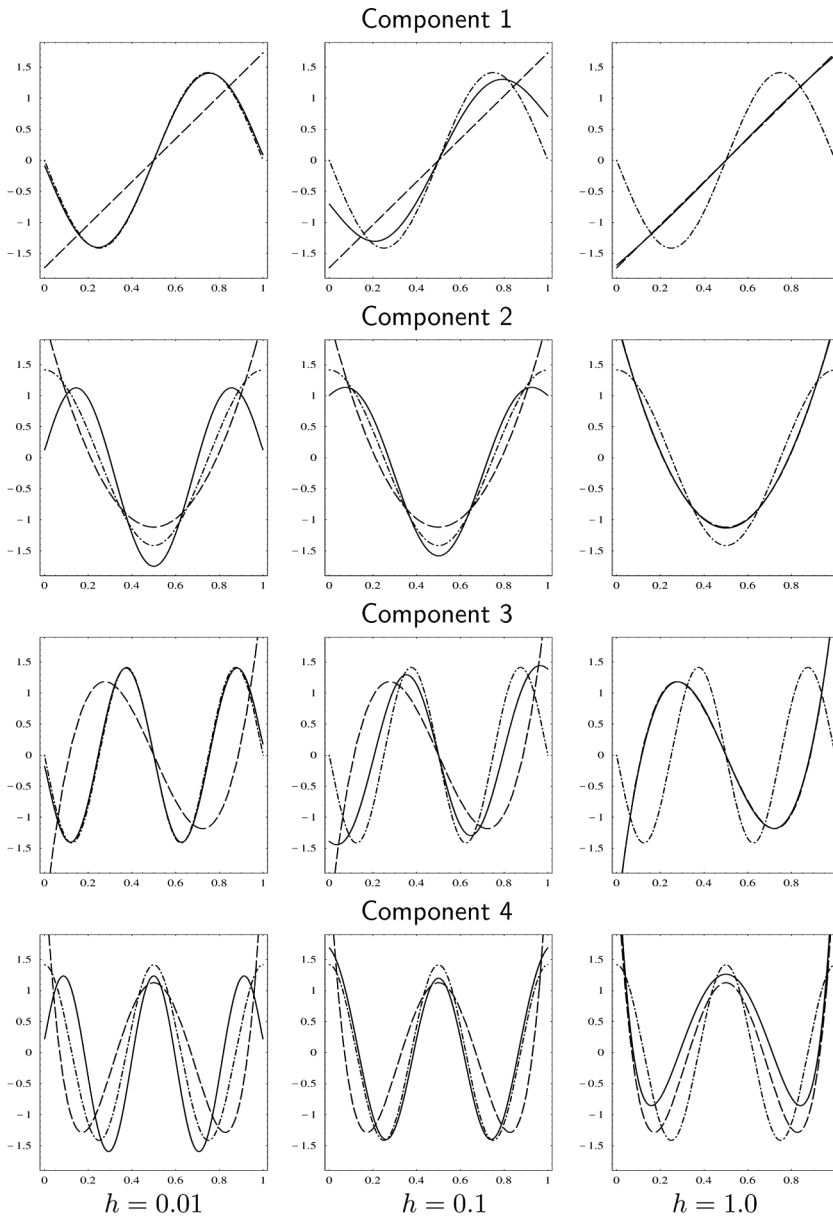
Figure 1. Principal components for: I_n^2(h) – solid line; A_n^2 – broken line; U_n^2 – broken and dotted line.
