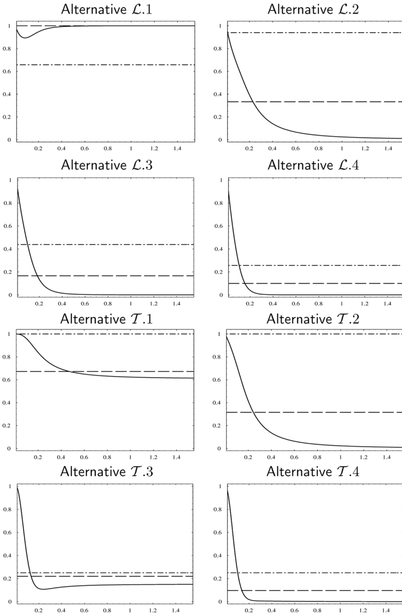
Figure 2. Local indices for Legendre and trigonometric alternatives as function of h : I_n^2(h) – solid line; A_n^2 – broken line; U_n^2 – broken and dotted line.
