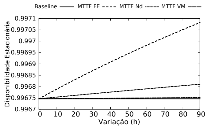
(b) MTTF
