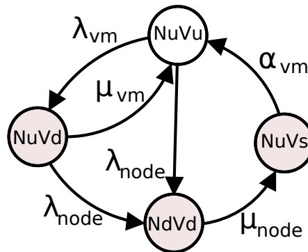
Figura 4.4: CTMC CloudNode
