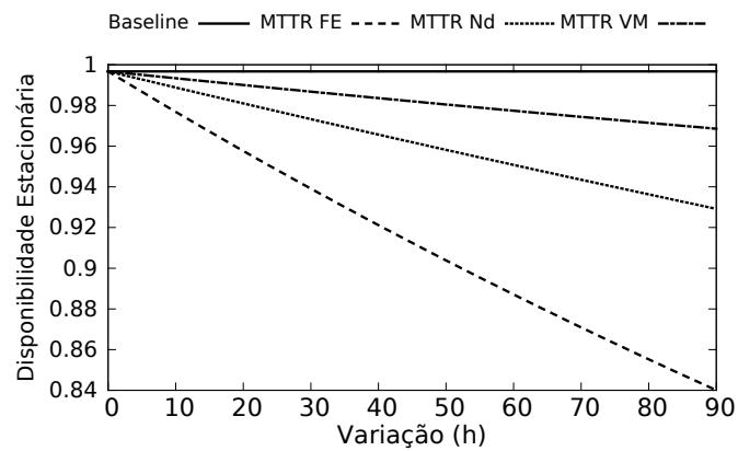
(c) MTTR
