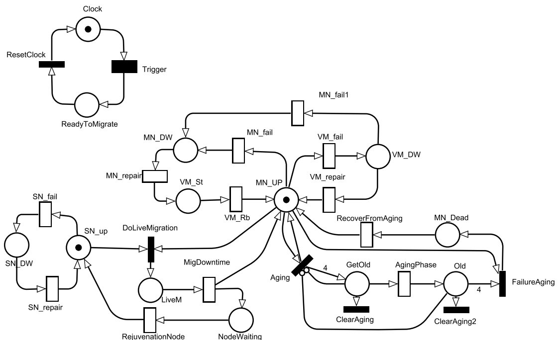
Figura 5.3: eDSPN CloudNodes
