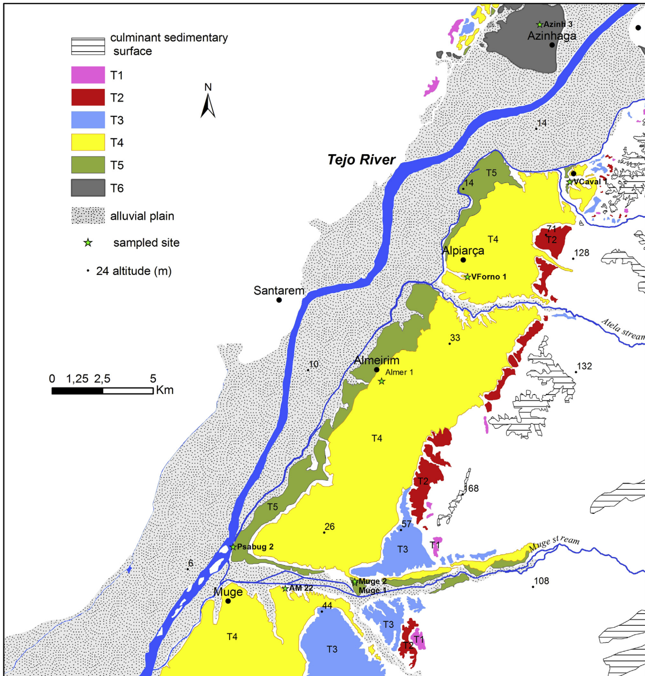
Fig. 3. Terrace staircase of the River Tejo reach IV. The T6 terrace is only visible near Azinhaga village, whilst T5 is buried by modern alluvium downstream of Muge. Note the asymmetric development of the terraces between the two sides of Tejo valley downstream of Chamusca. Terraces are very scarce on the west side of the river valley.
