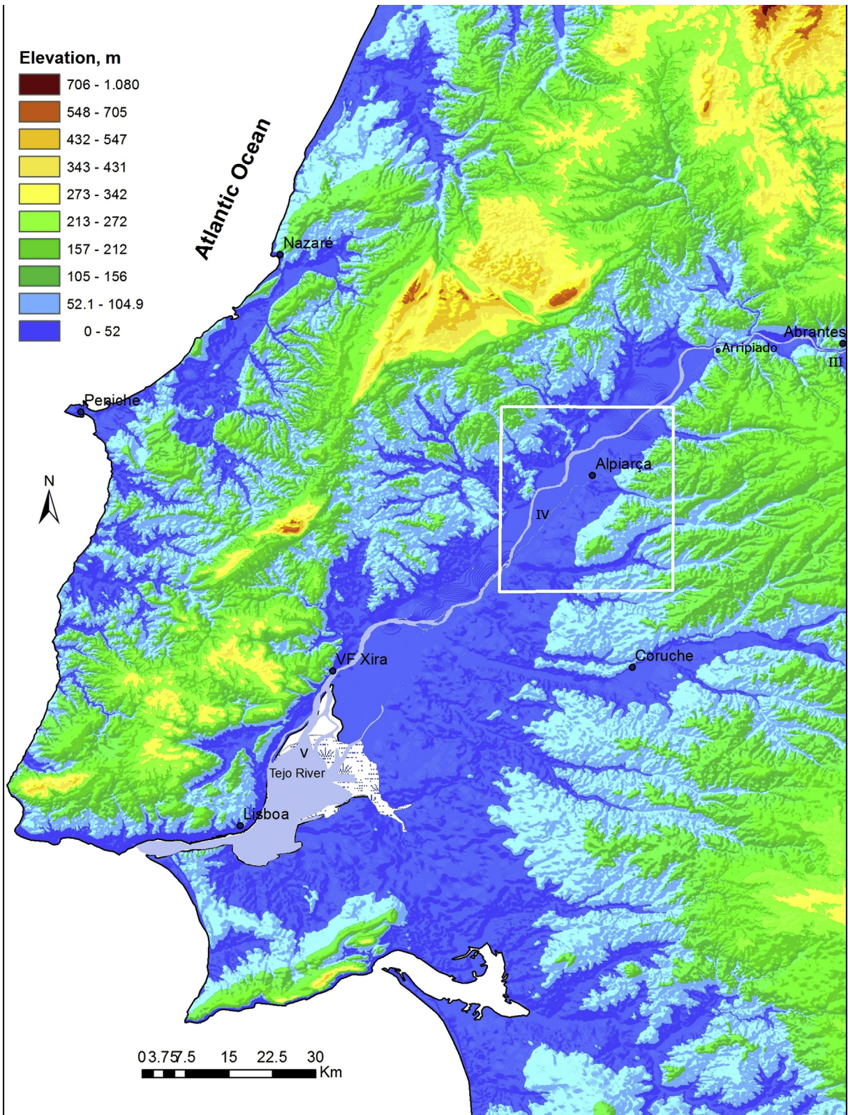
Fig. 1. Location of the study area in the Lower Tejo (central Portugal). Hypsometry and digital elevation model obtained from SRTM data. Several reaches of the Lower Tejo are shown: the distal part of the E-W oriented reach III (Abrantes); the NE-SW oriented reach IV (Arripiado – Alpiarça – Vila Franca de Xira); the reach V ( Vila Franca de Xira – Atlantic coast; the modern estuary).
