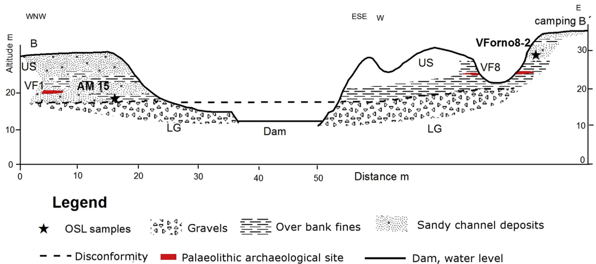
Fig. 6. Stratigraphic cross section B – B'. This section shows that the US unit is dominated by sand channel facies in the west and rich in flood-plain clayish silts in the east. The topographic position of sample AM 15 is at near distance from the cross section (see Fig. 4), in the west side of the Vale do Forno streamlet.
