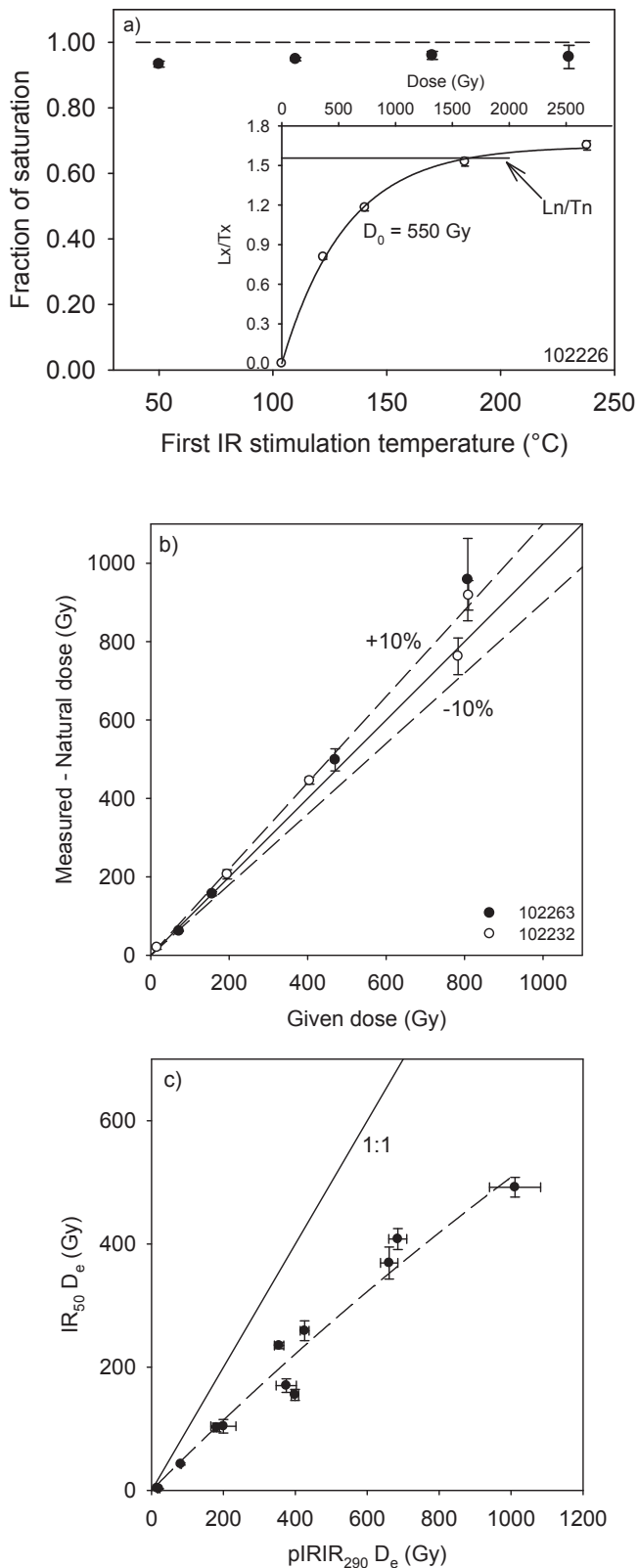
Fig. 15. a) First IR stimulation plateau for sample 102226. The natural signals are expressed as a fraction of the saturation level of the dose response curve. Three aliquots were measured per temperature and error bars represent one standard error. The inset shows the sensitivity corrected natural pIRIR290 signal (horizontal solid line) interpolated on the dose response curve for one aliquot measured using a first IR stimulation temperature of 50 °C. b) Results of the dose recovery measurements. At least three aliquots were measured per data point and error bars represent one standard error. c) IR 50 D e values plotted as a function of the pIRIR 290 D e values for
