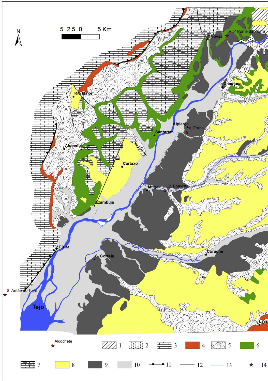
Fig. 2. Simplified geological map of the region (adapted from the Carta Geológica de Portugal, 1/500,000, Oliveira et al., 1992 and Barbosa, 1995). 1 – metasediments of the Hesperian Massif; 2 – granites of the Hesperian Massif; 3 – limestones and sandstones (Mesozoic); 4 – sandstones and conglomerates (Paleogene); 5 – sands (Lower Miocene); 6 – silts and clays (Miocene); 7 – limestones, silts and clays (Miocene); 8 – gravels and sands (Pliocene); 9 – gravels of fluvial terraces (Pleistocene); 10 – modern alluvium: mud, silt and sand (Holocene); 11 – thrust fault; 12 - fault; 13 - stream; 14 – archaeological site.
