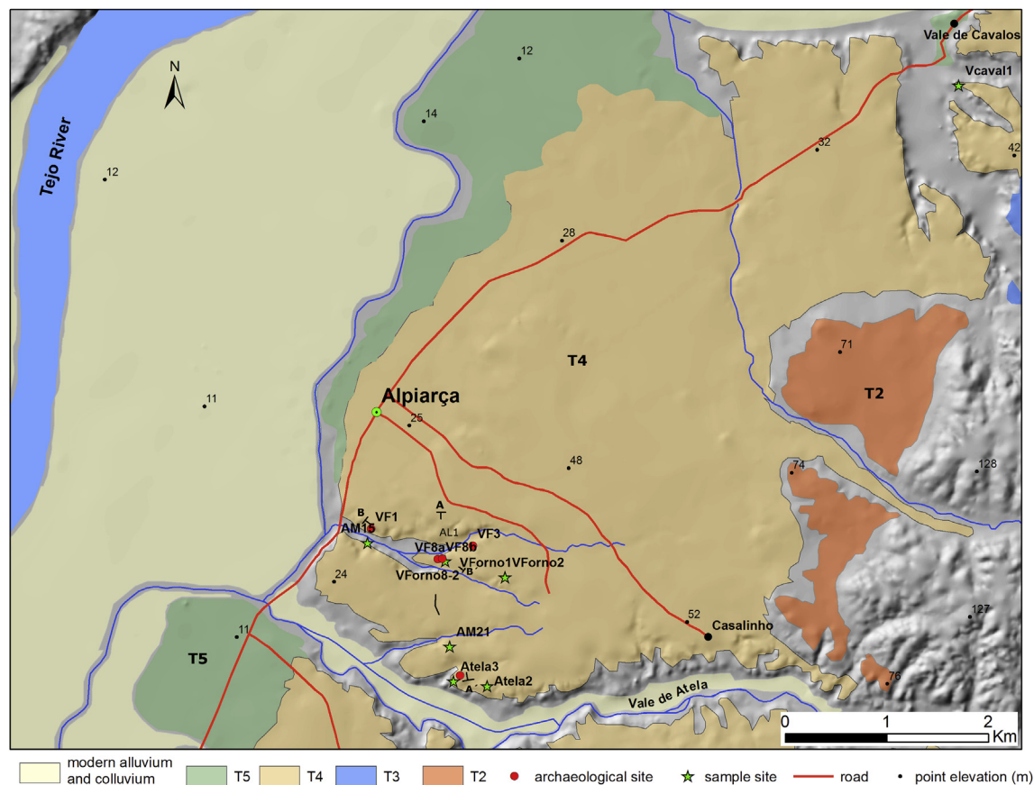
Fig. 4. Map of the Alpiarça area, comprising the River Tejo tributary valleys of Vale do Forno and Vale de Atela. Location of the sites and cross sections (A – A' and B – B'). It is deduced from the contour lines that the interfluvies between the Vale do Forno and Vale de Atela is developed in eroded (dissected) uppermost T4 deposits.
