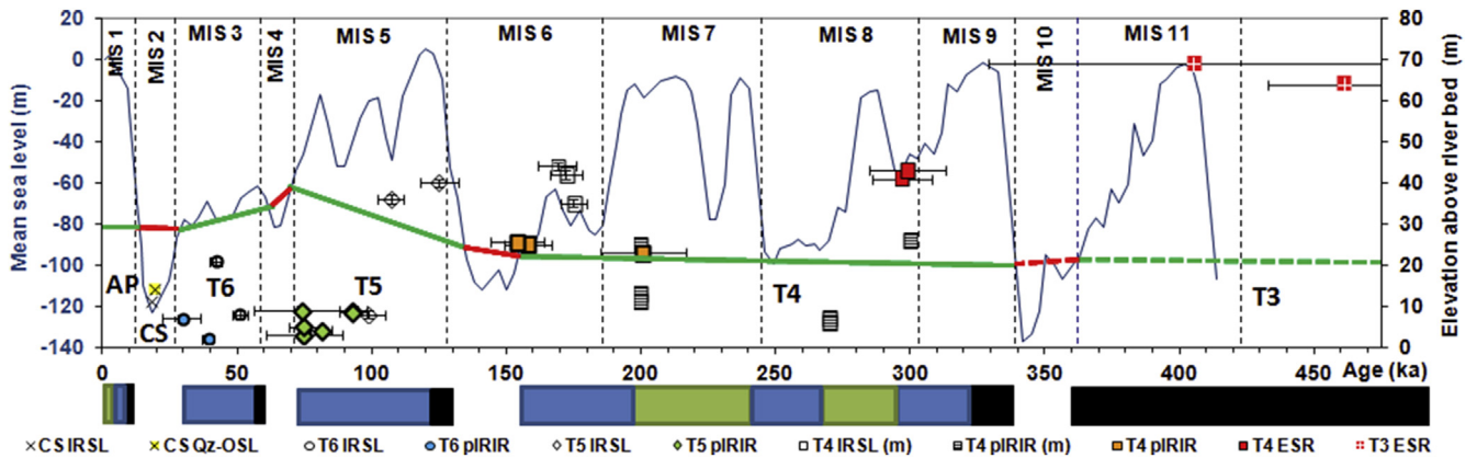
Fig. 17. Burial ages of samples collected from Middle to Late Pleistocene sedimentary units of the Tejo reach IV, plotted according to the respective elevation a.r.b. (right axis). Horizontal bars indicate the dominant lithologies for the fluvial deposits (black – gravels; blue – sands; green – silty clays) and the probable age range of each sedimentary unit. For this reach, the periods of aggradation are represented by green line segments and the periods of river downcutting are represented by red line segments that cross the sea-level curve (scaled benthic isotopes from V19–30, after Cutler et al., 2003), testifying a dominant sedimentary control by glacio-eustasy. T3, T4, T5 and T6 – terraces; CS – Carregueira Formation (aeolian sands); AP – Alluvial plain deposits. MIS intervals are according to Lisiecki and Raymo (2005). ESR – Electron Spin Resonance age; pIRIR – post-IR IRSL 290 SAR age (m – minimum age); IRSL – IRSL 50 SAR age (m – minimum age); Qz-OSL – Quartz OSL SAR age. (For interpretation of the references to colour in this figure legend, the reader is referred to the web version of this article.)
