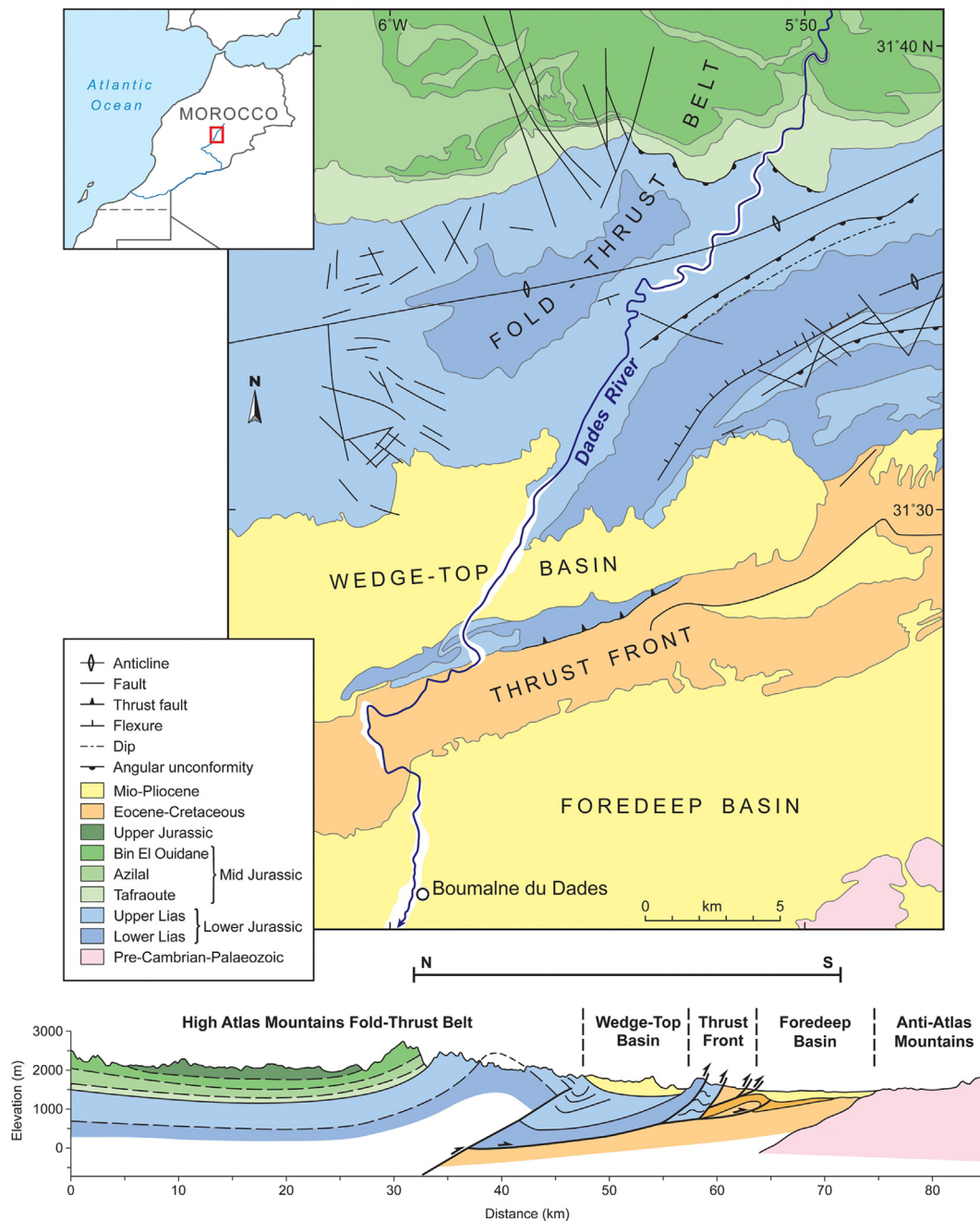
Fig. 2. A) Geology of the study area within the High Atlas orogenic system, illustrating key lithostratigraphic units and major tectonic and stratigraphic structures. B) North-South orogenic cross-section. Map and cross-section modified from Carte Géologique du Maroc (1975, 1990; 1993). See Table 1 for stratigraphic and lithologic information.
