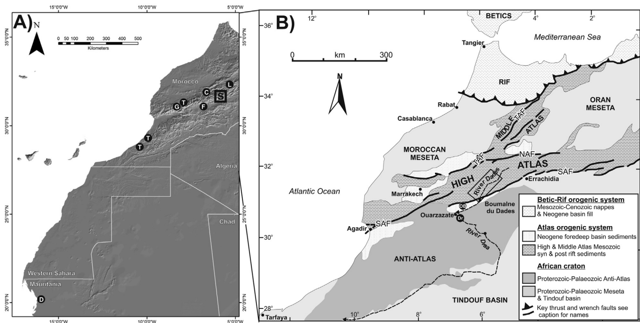
Fig. 1. A) Topography of NW Africa and Quaternary landscape study locations referred to within text (D = dune studies; T = terrace studies; G = glacier moraine study; F = fan studies; C = glacial cirque study; S = Dadès River study area; L = mountain lake study). B) Tectonic and geological configuration of Morocco and the south-central High Atlas region. Note River Dadès study region (black rectangle: Figs. 2 and 3). OB = Ouarzazate Basin; Dr = Draa gorge and capture region; NAF/SAF/TAF = Northern/Southern/Tell Atlas Fault systems. Modified from Michard (1976) and Carte Géologique du Maroc (1985).
