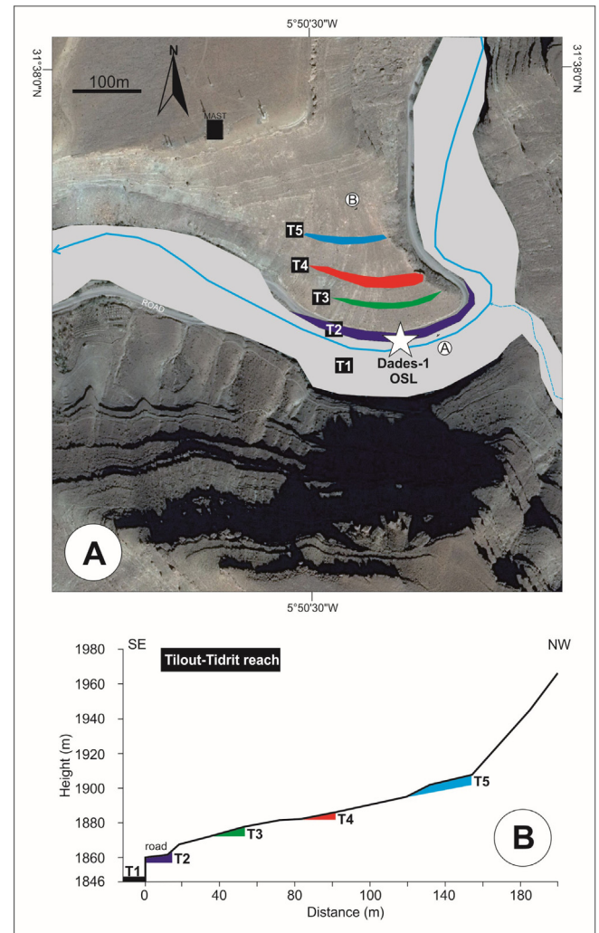
Fig. 7. Map (A) and topographic profile (B) of T1-T5 terrace staircase, upstream FTB region terrace staircase. See Fig. 8E and Supplementary Information for OSL sample information.
