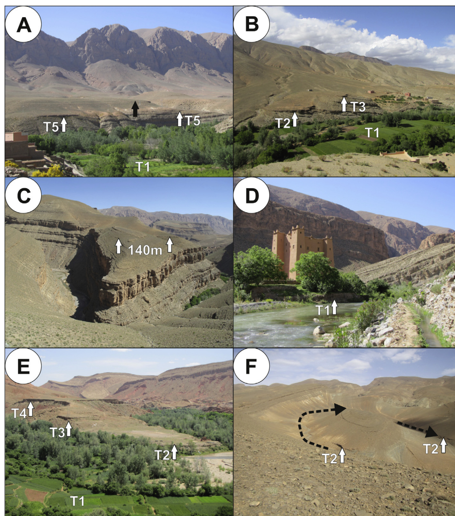
Fig. 6. River terrace field imagery: A) Laterally extensive T5 terrace levels (white arrows) buried by tributary fan slope sediments (black arrow), mid FTB region. B) T2-T3 terrace level remnants, inset by large relict tributary fan, mid FTB region. C) The highest documented terrace level remnants at 140m, proximal FTB region. D) T1 terrace level (arrow) ~2 m above modern river, immediately upstream of Tarhía n' Dadès gorge, distal FTB region. E) Well developed T1-T4 terrace staircase, downstream TF region. F) Abandoned bedrock meander containing T2 upstream-downstream terrace remnants buried by locally derived slope deposits, proximal FTB region.
