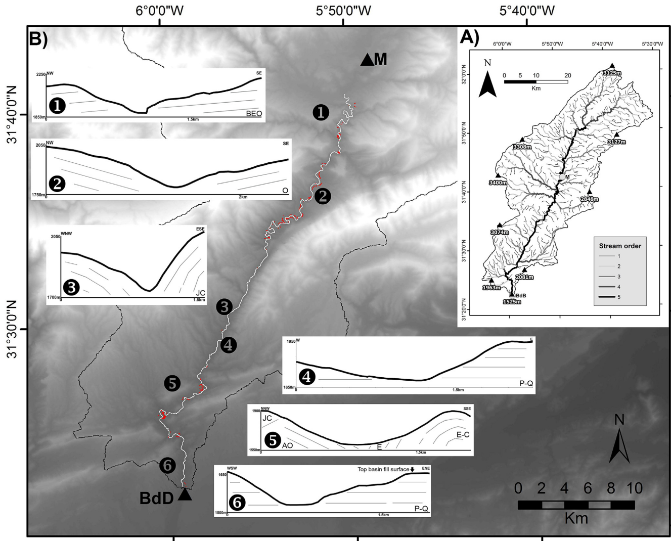
Fig. 3. A) Dadès River catchment, relief and Strahler stream ordering. B) Detailed study area showing the drainage divide (black line), the Dadès River trunk drainage study region (white line) between the towns of Boumalne du Dadès (BDD) and M'smerir (M), river terrace distribution (red dots) and cross valley profiles (1–3 = proximal, mid, distal FTB; 4 = WTB; 5 = TF; 6 = FB) annotated with geology and regional bedrock dip configuration (P-Q = Plio-Quaternary; AO = Ait Ouglif Fm; E-C = Eocene-Cretaceous; BEO = Bin El Ouidane Fm, O = Ouchbis Fm, JC = Jbel Choucht Fm; See Fig. 2 and Table 1).
