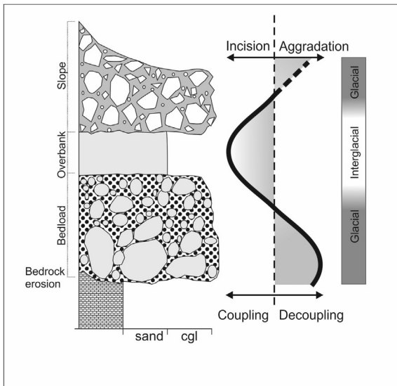
Fig. 11. A conceptual river terrace-climate model for the Dadès River illustrating the relationship between glacial-interglacial climates, valley floor incision-aggradation patterns and river channel-hillslope coupling status.
