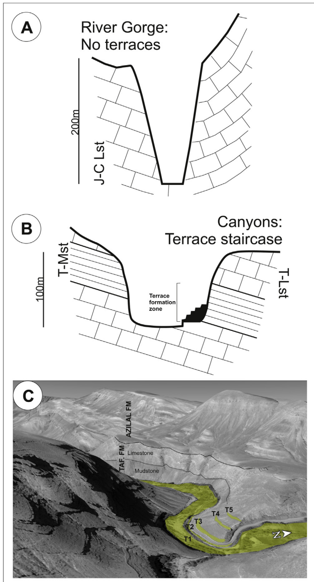
Fig. 10. A) River gorge reach of structurally thickened ‘strong’ limestone with no terrace formation. B) Confined canyon reach where river terrace staircase development is controlled by the strength variability in a dipping stratigraphic sequence of Taфраoute Fm mudstone (T-Mst) and limestone (T-Lst). C) Oblique Google Earth image illustrating rock strength, structure and stratigraphic sequence relationships to terrace staircase formation at the Tilout site (Fig. 7).
