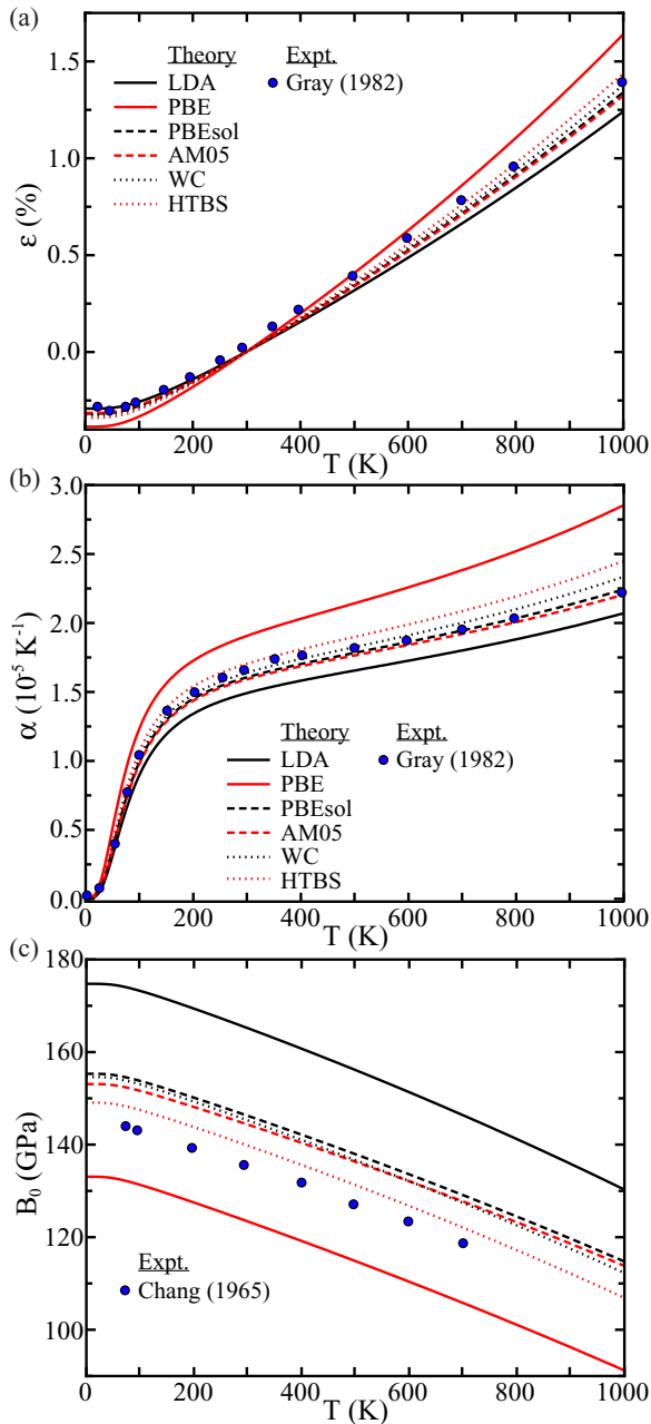
FIG. 11. (Color online) Variation of (a) the linear thermal expansion \epsilon , (b) the coefficient of linear thermal expansion \alpha , and (c) the bulk modulus B_0 of copper as a function of the temperature computed using the different XC functionals: LDA in solid black, PBE in solid red (gray), PBEsol in dashed black, AM05 in dashed red (gray), WC in dotted black, and HTBS in dotted red (gray). Relevant experimental data are reported. The labels correspond to the first author and year of publication of Refs. [65,66].
