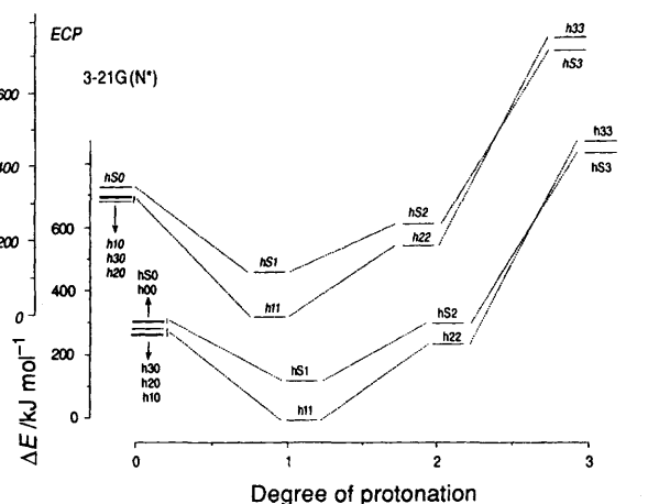
Fig. 5 Representation of the energy difference between the different conformers found for the [9]aneN 3 amine through the corresponding protonation process. Comparison between the ECP and the 3-21G(N*) results.
