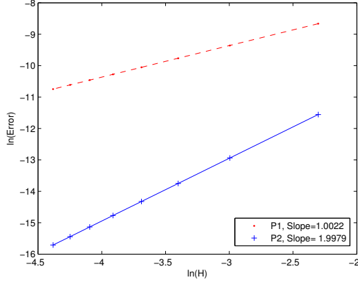
Figure 1: \ln(\|\tilde{c} - \tilde{c}_H\|_{H^1(\Omega, \mathbb{C}_\sigma^+)}) versus \ln(H) .
