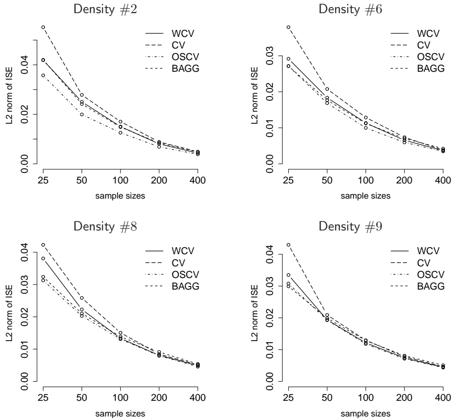
Figure 2: Empirical L^2 -norm of \text{ISE}(f; n, \hat{h}) associated to the bandwidth selector methods WCV, CV, OSCV and BAGG, for some “easy-to-estimate” densities. The number of replications is 500.
