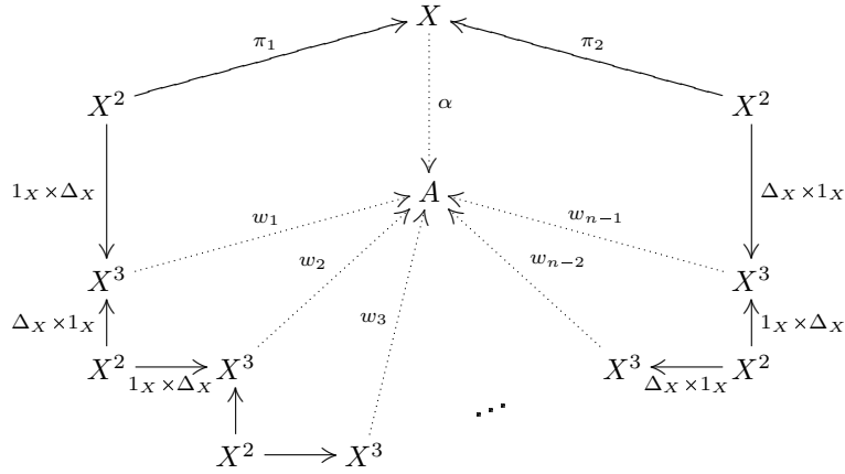
FIGURE 1. Approximate Hagemann–Mitschke operations
