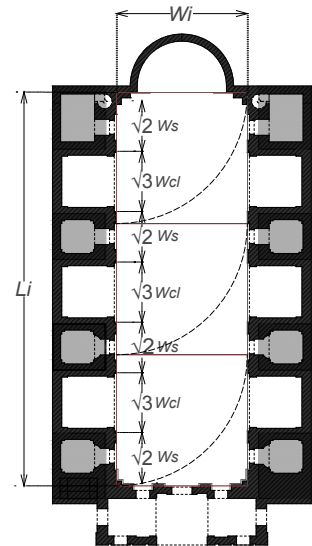
5. Sant'Andrea's plan summarizing the analysis of cell proportions; the skeleton between lateral chapels proportions; the rooms that fill space between chapels.
