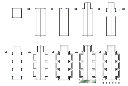
4. Computation of a design solution similar to the church of São Vicente de Fora.
