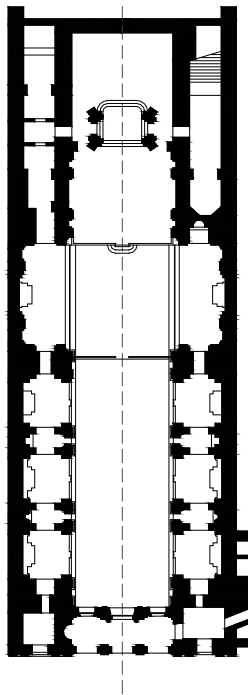
3. Plan of São Vicente de Fora church.
