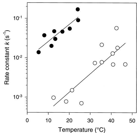
Fig. 3. Temperature dependency of the proton permeability of liposomes prepared from lipids derived from B. subtilis cells grown at 13°C (●) and 50°C (○). The influx of protons, as measured with the fluorescent probe pyranine, was fitted to a first-order kinetic equation as described in Section 2.
