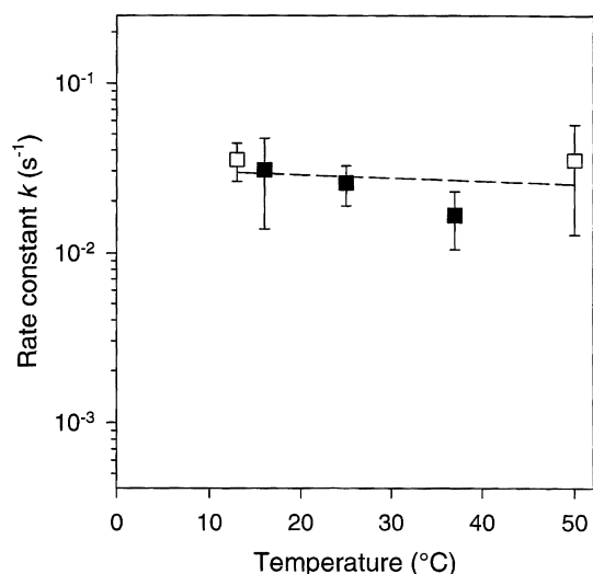
Fig. 4. Proton permeability at the growth temperature of liposomes prepared from lipids derived from B. subtilis cells grown at temperatures between the lower and upper temperature limit (■ ± S.D., n \geq 3 ). Inter- and extrapolation of the exponential fit on growth temperature curves at 13°C and 50°C, shown in Fig. 3 (□ ± 95% confidence intervals). The influx of protons, as measured with the fluorescent probe pyranine, was fitted to a first-order kinetic equation as described in Section 2.
