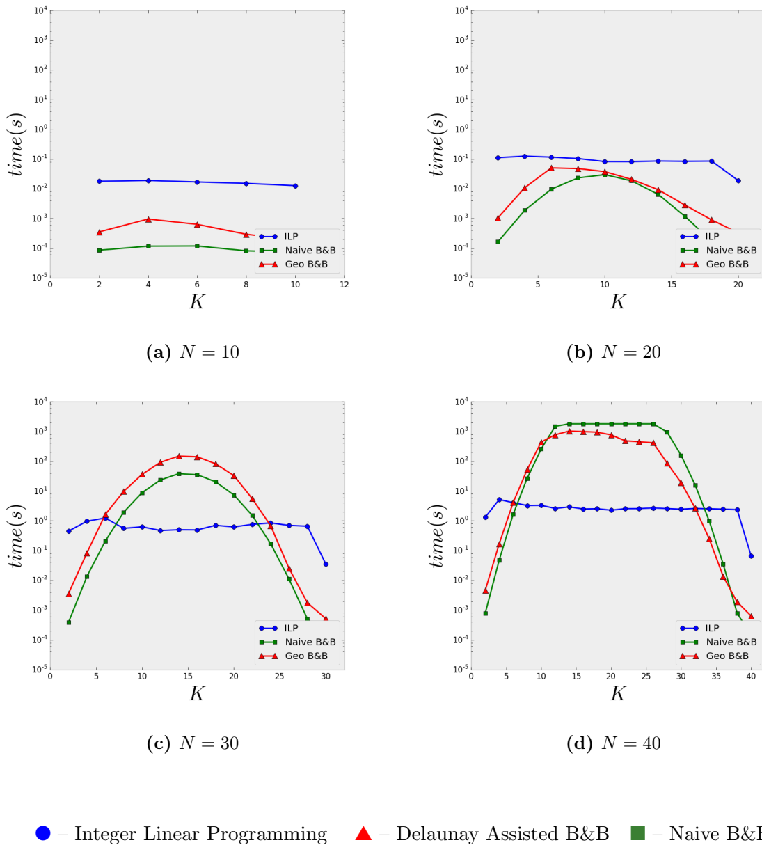
Figure 3.12. CPU-time for different values of N with varying values of K
