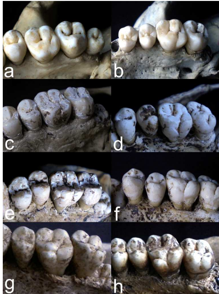
Figure 2. Different expressions of Carabelli's trait, according to ASUDAS: a) smooth mesiopalatal surfaces on the first (UM1) and second upper molars (grade 0; note also the reduced third molar); b) slight diagonal groove on the palatal surface of the mesiolingual cusp of UM1 (grade 1); c) mesiolingual cusp of UM1 indentation on the most occlusal and mesial corner of the lingual facet (grade 2, darkened post mortem ; note forming third molar) ; d) ASU grade 3 (small Y shaped groove); e) grade 4 (deeper and larger Y shaped groove); f) grade 5 (small mesiolingual cusp; g) grade 6; h) grade 7. Images d, e, g and h are from the right side of the upper dental arcade. Images a, b, c and f are from the left side.
