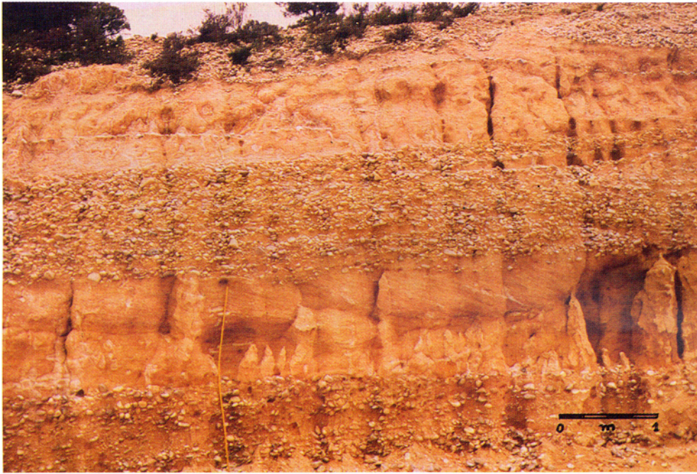
Photo 3 — Serra de Almeirim Conglomerates: barforms near Almeirim, with mean maximum particle sizes (MPS) = 20 cm.
