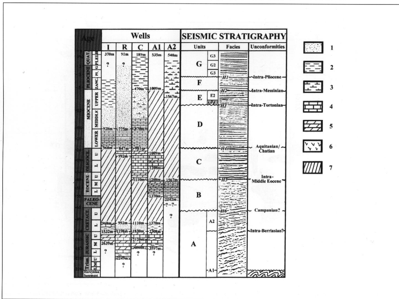
Fig. 2. Seismic stratigraphy, main unconformities and wells of the Algarve offshore. I: Imperador-1; R: Ruivo-1; C: Corvina-1; A1: Algarve-1; A2: Algarve-2. Wells lithologies: 1: sands; 2: clays; 3: silts; 4: limestones; 5: dolomites; 6: evaporites; 7: hiatus
