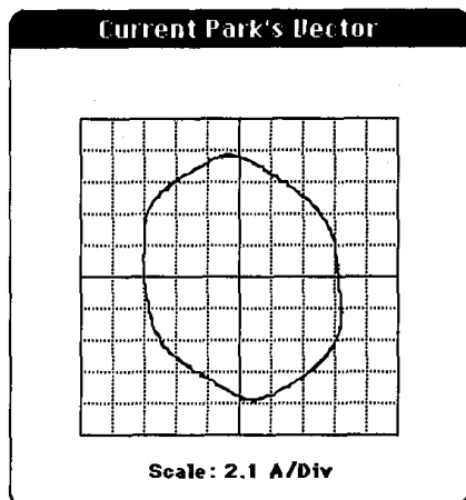
Fig. 5 — Experimental current Park's Vector pattern, for the case of six shorted turns in phase A ( U_3-U_4 ).
