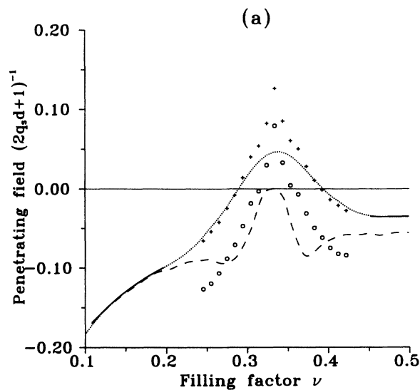
FIG. 1. Penetration field (1+2q_d)^{-1} vs filling factor \nu . Solid lines show the result of computer simulation, dotted lines obtained in NGA. Dashed line shows the experimental data from Ref. 10. Magnetic field for the plot is 12 T.
