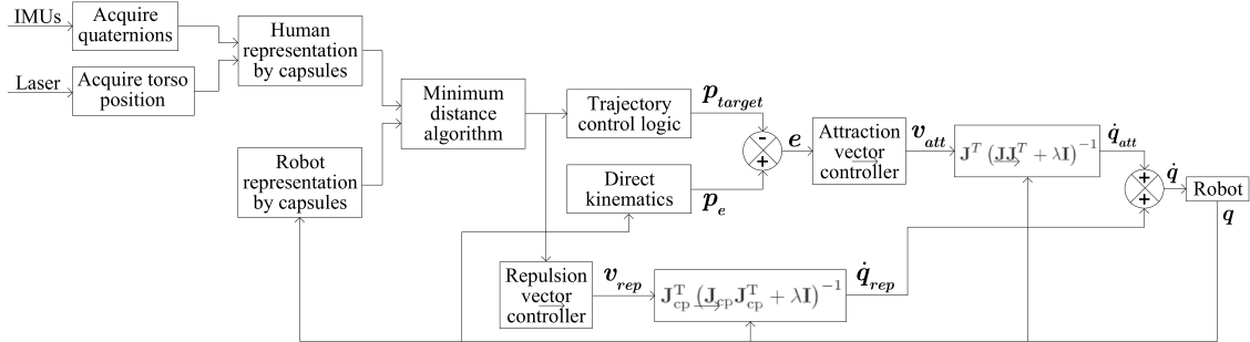
Fig. 8. Collision avoidance general architecture.
