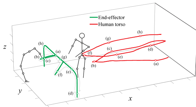
Fig. 12. Robot end-effector path and the human torso trajectory related to experimental tests (Experiment 1) in Fig. 10, points (a)–(h). It is possible to visualize that the robot path is modified when the human approaches the robot and then the robot returns back to the nominal path. The human approaches the robot twice, to place the box on the table and to take the screwdriver from the table.
