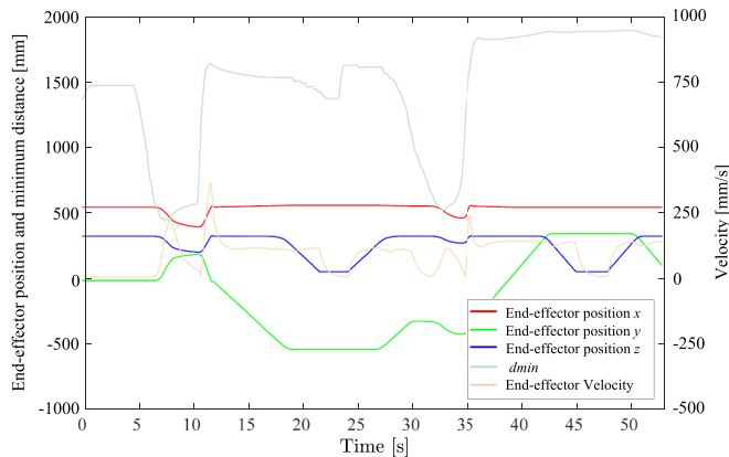
Fig. 11. Human-robot minimum distance, robot end-effector position and velocity recorded during Experiment 1.
