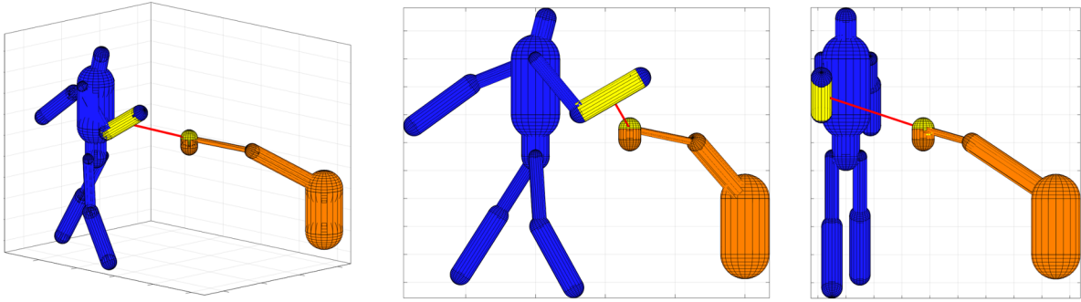
Fig. 7. Human-robot minimum distance visualization in MATLAB GUI.
