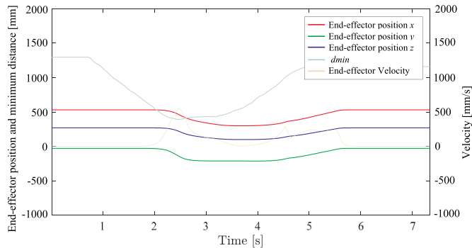
Fig. 14. Human-robot minimum distance, robot end-effector position and velocity recorded during Experiment 2.
