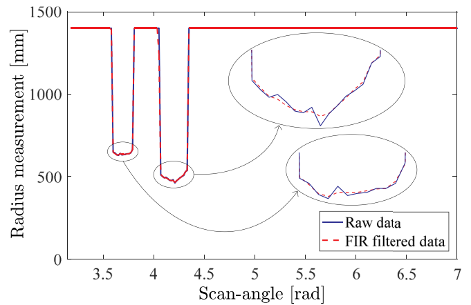
Fig. 3. Raw data and FIR filtered of radius measurement with scan-angle, close ups show filtered data are smoother in the critical parts of the curves.
