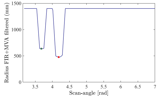
Fig. 4. Filtered radius measurement with scan-angle. Minima are marked with green and red dots representing the human legs. (For interpretation of the references to color in this figure legend, the reader is referred to the web version of this article.)
