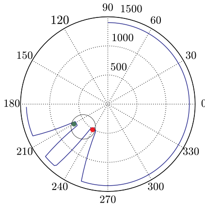
Fig. 5. Human legs detected in the laser scan field. Red and green dot represent the legs and the black circle represents the torso. (For interpretation of the references to color in this figure legend, the reader is referred to the web version of this article.)
