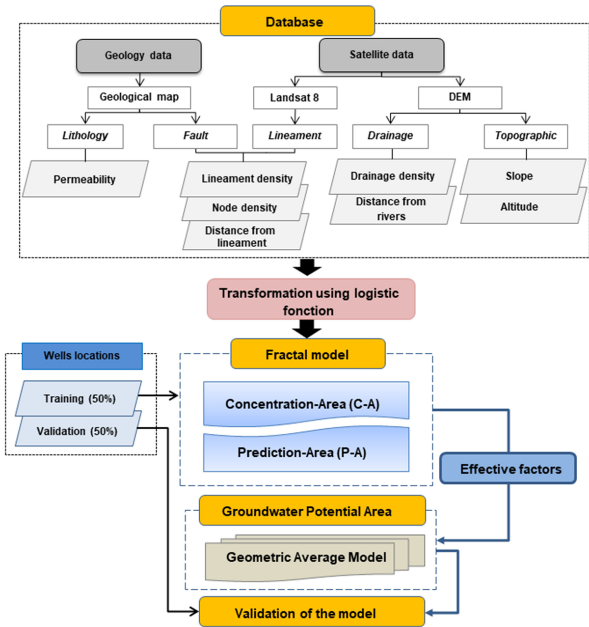
Figure 3. The methodology used for editing the potential groundwater map for the Tissent basin.
