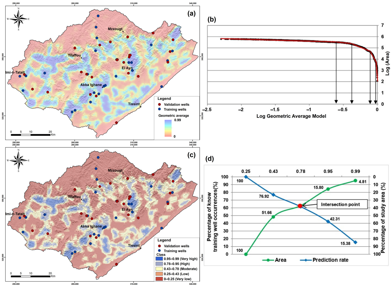
Figure 8. (a) Groundwater potentiality map of Tissint basin using the geometric average model; (b) Concentration-area (C-A) log-log plots of G_{A\ GWPA} ; (c) Classified map of G_{A\ GWPA} ; (d) Prediction-area (P-A) plot for the classed map of G_{A\ GWPA} .
