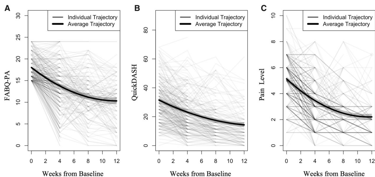
Figure 3. Longitudinal trajectories across time. (A) FABQ-PA; (B) QuickDASH; (C) Pain level. Lighter lines represent individual trajectories (with darker lines meaning overlap of trajectories), while average trajectories calculated through LGCA are depicted in bold lines, with shadowing representing 95% confidence intervals. LGCA = latent growth curve analysis.
