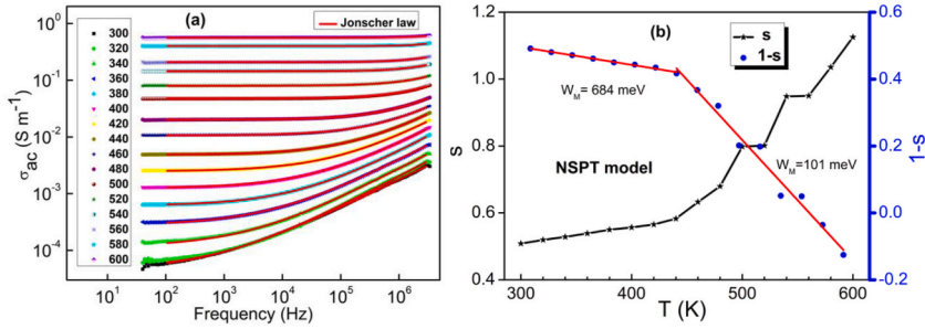
Fig. 4. (a) Frequency response of ac conductivity at several temperatures and (b) Temperature dependence of s and 1-s of \text{Cu}_{0.5}\text{Fe}_{2.5}\text{O}_4 .
