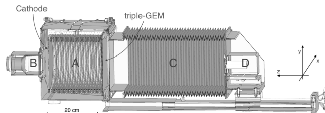
Fig. 1. The LEMOn prototype [4]. The elliptical sensitive volume (A), the PMT (B), the optical bellow (C) and the sCMOS camera (D) are indicated.
