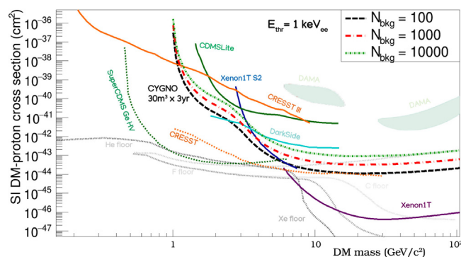
Fig. 2. Spin Independent 90% CI for WIMP-nucleon cross section for 30 m 3 CYGNO detector for 3 years of exposure with different background level assumptions and operative threshold of 1 keV ee .
