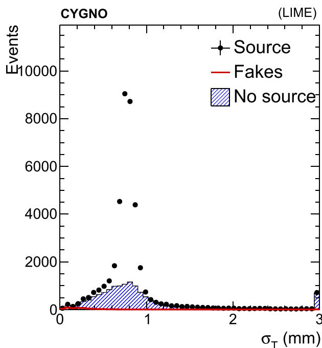
Fig. 9 Top: light density \delta in the reconstructed clusters, as defined in the text. Bottom: transverse dimension of the reconstructed cluster \sigma_T . Black points represent data in presence of the ^{55}\text{Fe} source, filled histogram represents data without the source, while the red hollow histogram represents the contribution from mis-reconstructed clusters from electronics noise. The latter two are normalized to the live-time of the data taking with the ^{55}\text{Fe} source
