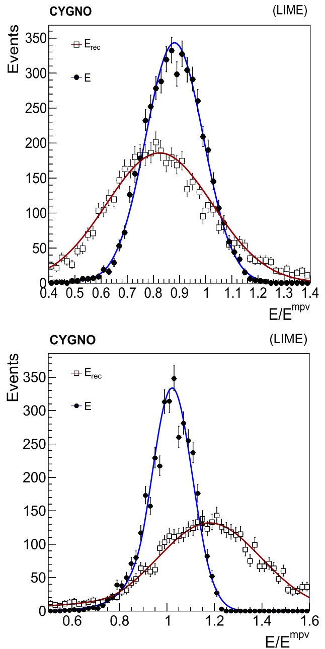
Fig. 13 Comparison between E_{rec} (open squares) and E (filled circles) normalized by the most probable value of the corresponding distribution for z = 25 cm, on data collected with ^{55}\text{Fe} source at a distance of z = 10 cm (top) or z = 40 cm (bottom) from the GEM planes. A fit with a Crystal Ball function, as described in the text, is superimposed to each distribution
