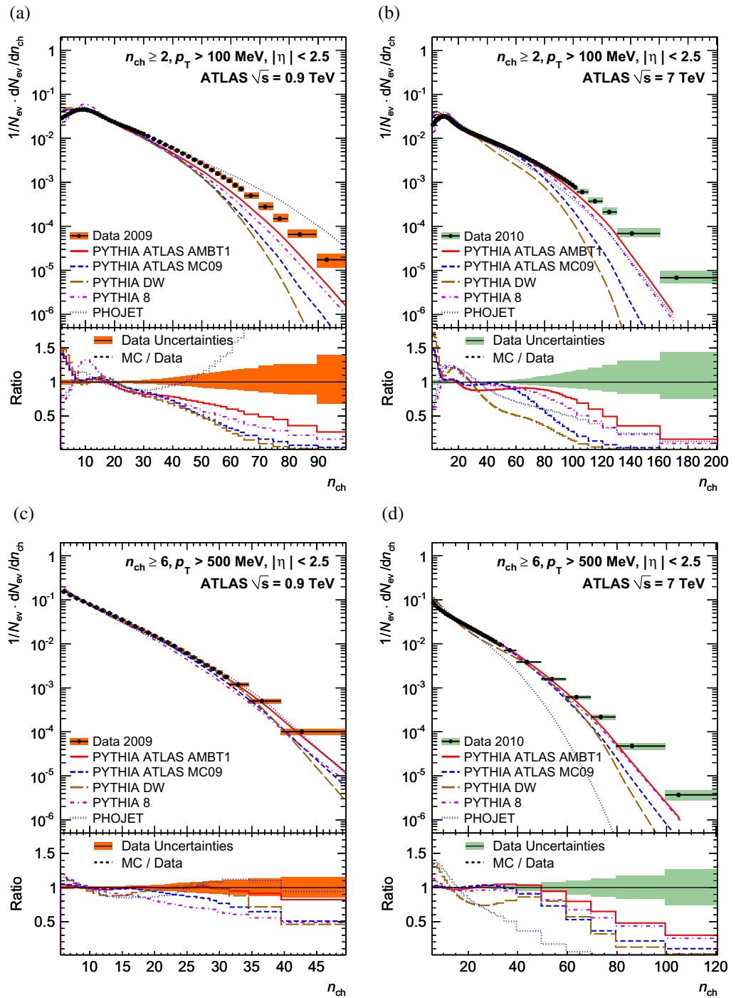
Figure 10. Charged-particle multiplicity distributions for events with n_{ch} \geq 2 , p_T > 100 MeV (a, b) and n_{ch} \geq 6 , p_T > 500 MeV (c, d) and |\eta| < 2.5 at \sqrt{s} = 0.9 TeV (a, c) and \sqrt{s} = 7 TeV (b, d). The dots represent the data and the curves the predictions from different MC models. The vertical bars represent the statistical uncertainties, while the shaded areas show statistical and systematic uncertainties added in quadrature. The bottom insets show the ratio of the MC to the data. The values of the ratio histograms refer to the bin centroids.
