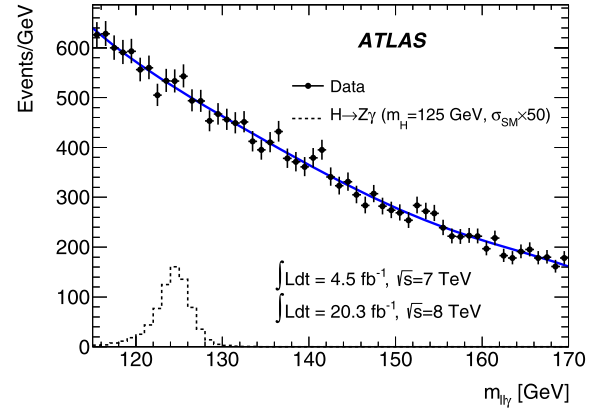
Fig. 2. Distribution of the reconstructed \ell\ell\gamma invariant mass in data, after combining all the event categories (points with error bars). The solid dark grey (blue in the web version) line shows the sum of background-only fits to the data performed in each category. The dashed histogram corresponds to the signal expectation for a Higgs boson mass of 125 GeV decaying to Z\gamma at 50 times the SM-predicted rate.
