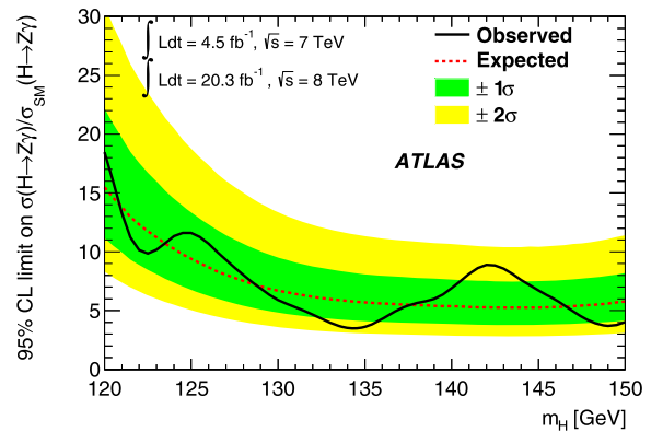
Fig. 3. Observed 95% CL limits (solid black line) on the production cross section of an SM Higgs boson decaying to Z\gamma divided by the SM expectation. The limits are computed as a function of the Higgs boson mass. The median expected 95% CL exclusion limits (dashed red line), in the case of no expected signal, are also shown. The green and yellow bands correspond to the \pm 1\sigma and \pm 2\sigma intervals. (For interpretation of the references to colour in this figure legend, the reader is referred to the web version of this article.)
