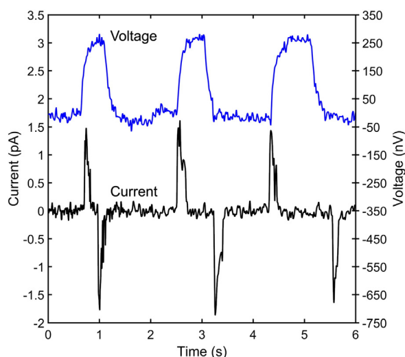
Fig. 10. Time trace of current and voltage spikes observed on a culture of C6 glioma cells. The data was recorded using gold electrodes with a width of 100 \mu\text{m} . The electrodes are of type B as described on Table 1.
