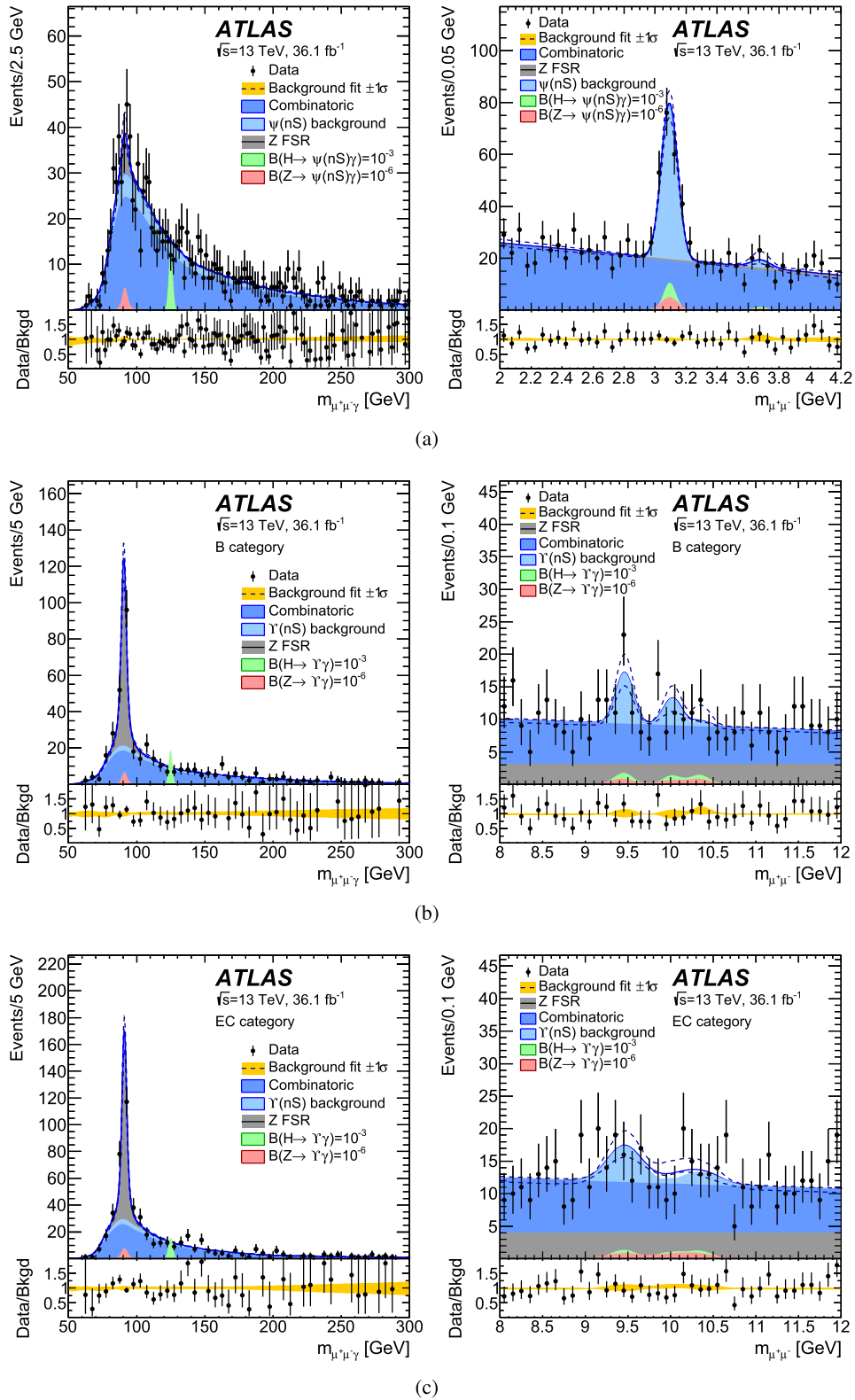
Fig. 4. The m_{\mu^+\mu^- \gamma} and m_{\mu^+\mu^-} distributions for the selected (a) \psi(nS)\gamma and \gamma(nS)\gamma ((b) barrel and (c) endcap categories) candidates along with the results of the maximum-likelihood fits with background-only models. Z FSR refers to the Z \rightarrow \mu^+\mu^- \gamma background contribution. The solid blue line denotes the full fit result and the dashed blue lines correspond to its \pm 1\sigma uncertainty band. The ratios of the data to the background-only fits are also shown. (For interpretation of the colours in the figure(s), the reader is referred to the web version of this article.)
