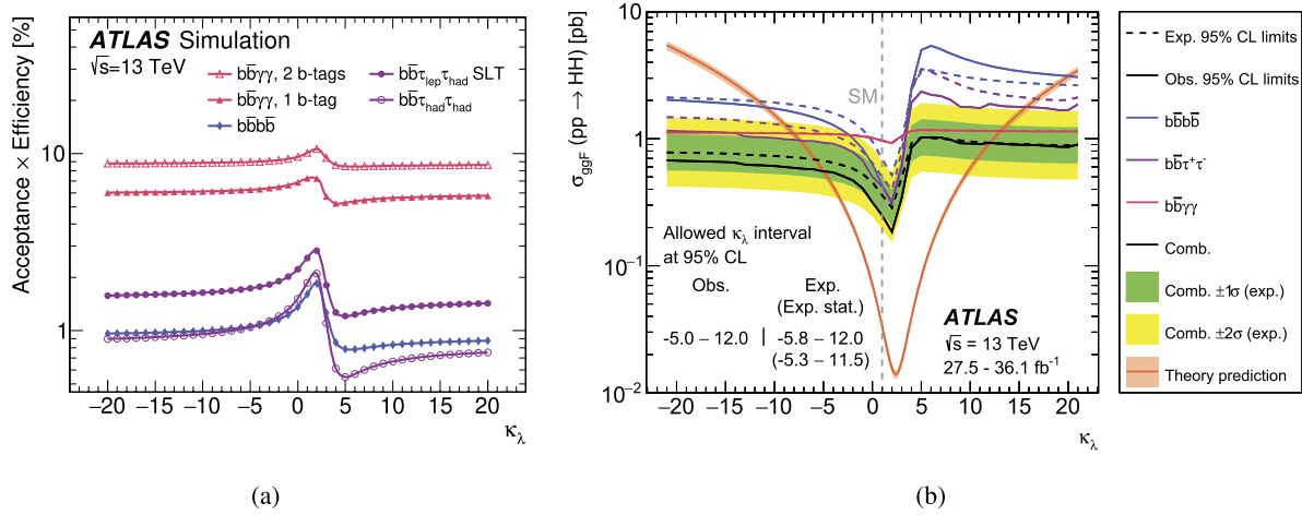
Fig. 4. (a) Signal acceptance times efficiency as a function of \kappa_\lambda for the b\bar{b}\bar{b}\bar{b} , b\bar{b}\tau^+\tau^- and b\bar{b}\gamma\gamma analyses. The b\bar{b}\bar{b}\bar{b} curve is the average of the 2015 and 2016 curves weighted by the integrated luminosities of the two datasets. (b) Upper limits at 95% CL on the cross-section of the ggF non-resonant SM HH production as a function of \kappa_\lambda . The observed (expected) limits are shown as solid (dashed) lines. In the b\bar{b}\gamma\gamma final state, the observed and expected limits coincide. The \pm 1\sigma and \pm 2\sigma bands are only shown for the combined expected limit. The theoretical prediction of the cross-section as a function of \kappa_\lambda is also shown. The effect of non-SM Higgs decay branching fractions due to \kappa_\lambda variations is not taken into account, which impacts the \kappa_\lambda intervals by no more than 7%.
