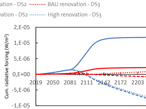
Figure 3. Cumulative radiative forcing for all end of life scenarios, comparing the business as usual (BAU) with the high renovation rate.
