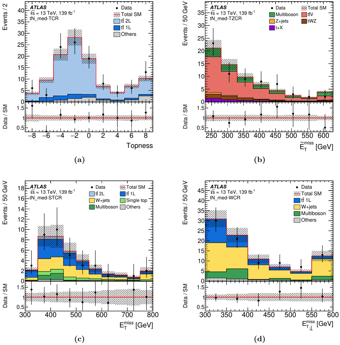
Figure 3. Selected kinematic distributions in tN_{med} CRs: (a) topness in the TCR, (b) \tilde{E}_T^{miss} in the TZCR, (c) E_T^{miss} in the STCR, (d) E_{T,\perp}^{miss} in the WCR. The distributions shown are post-fit, i.e. each background is scaled by a normalisation factor obtained from a background-only likelihood fit to the CRs (see table 14). The hatched area around the total SM prediction and the hatched band in the Data/SM ratio include all statistical and systematic uncertainties. The last (first) bin contains overflows (underflows).
