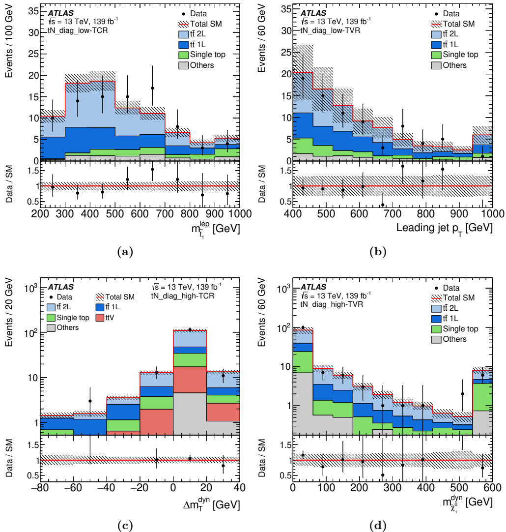
Figure 6. Selected kinematic distributions in tN_diag_low and tN_diag_high TCRs and TVRs: (a) m_{l_1}^{lep} in the tN_diag_low TCR, (b) leading jet p_T in the tN_diag_low TVR, (c) \Delta m_T^{dyn} in the tN_diag_high TCR, (d) m_{\chi_1^0}^{dyn} in the tN_diag_high TVR. The distributions shown are post-fit, i.e. each background is scaled by a normalisation factor obtained from a background-only likelihood fit to the CRs (see table 14). The hatched area around the total SM prediction and the hatched band in the Data/SM ratio include all statistical and systematic uncertainties. The last (first) bin contains overflows (underflows).
