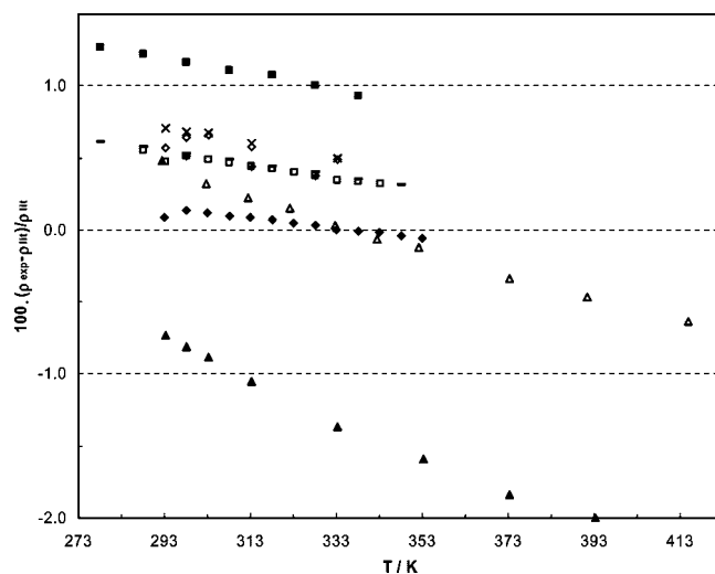
Figure 1. Relative deviations between the experimental density data of [C 2 mim][EtSO 4 ] at 0.10 MPa and those reported in the literature as a function of temperature at 0.10 MPa: \Delta , Jacquemin et al.; 5 \diamond , Hofman et al.; 20 \square , Gomez et al.; 31 - , Rodriguez et al.; 32 + , Gonzalez et al.; 33 \blacklozenge , Krummen et al.; 34 \blacksquare , Yang et al. 35 At 35.00 MPa: \blacktriangle , Jacquemin et al.; 5 \times , Hofman et al. 20
