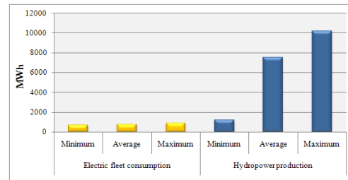
Figure 27: Electric fleet consumption and hydropower production
