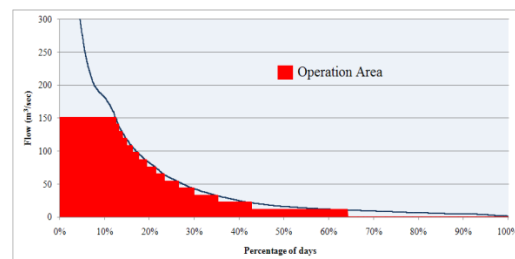
Figure 26: Small hydro operation area
