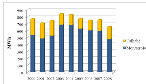
Figure 16: Annual consumption of trolleybus traction lines
