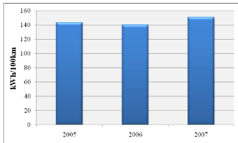
Figure 19: Electric mini-buses annual average consumption
