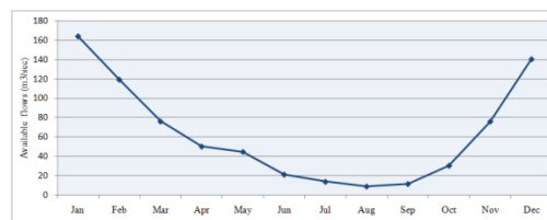
Figure 23: Monthly average of the average daily flows available for the production of energy
