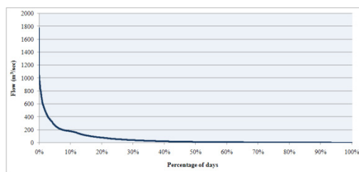
Figure 25: Coimbra dam-bridge flow duration curve
