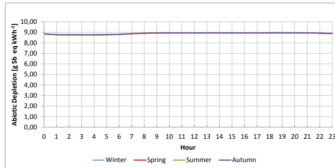
(a) 2011 Polish Electricity Mix
