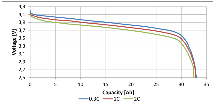
Figure 2: Capacity variation for several discharge profiles, for a Nissan Leaf battery pack cell, under different loads. For a fresh cell, under a discharge current of 0.3C the cell can store 32.5 Ah [33].
