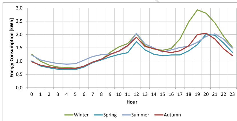
Figure 5: Seasonal variation in the load diagram for the household during the second life of batteries [44].
