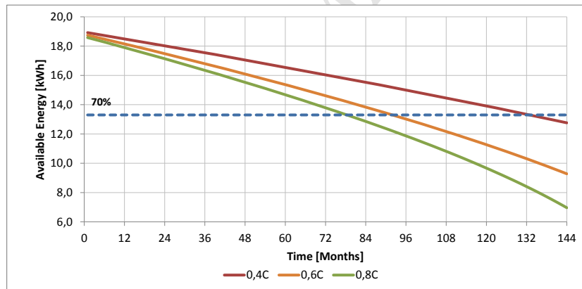
Figure 3: Capacity loss over time for an initial available capacity of 19 kWh (24 kWh in total) for different discharge rates.
