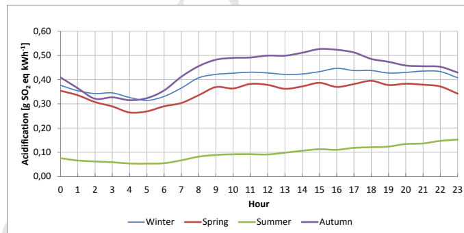
(c) French Electricity Mix
