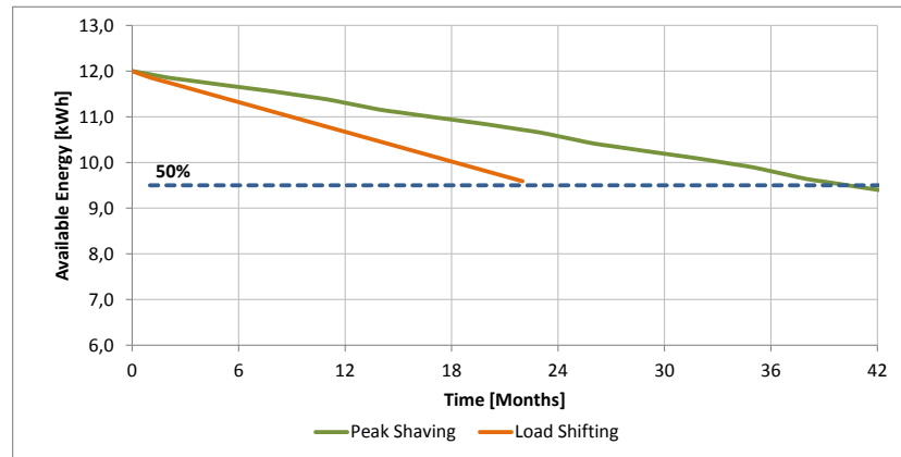
Figure 6: Storage capacity available over time for the second life of a electric mobility battery pack used in a peak shaving and load shifting application. For the second life, the battery pack has an initial capacity of 13 kWh, from which on only around 12 kWh are available, taking into account the discharge efficiency. The battery is no longer suitable when the capacity drops to 9.5 kWh (50% of the initial available capacity).
