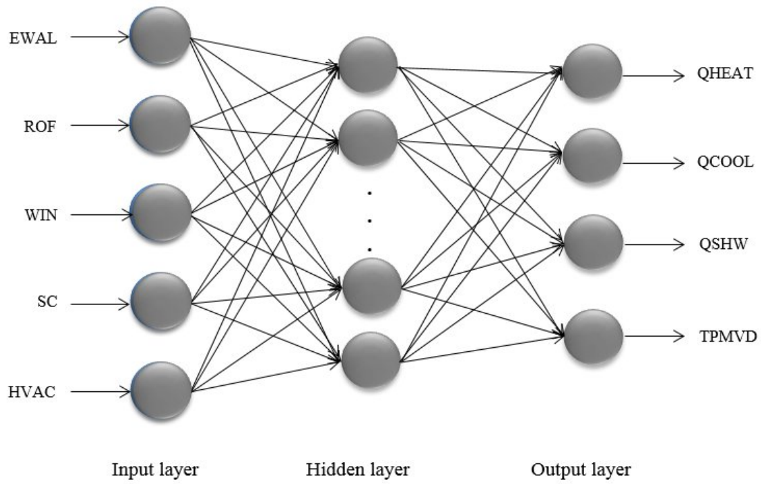
Figure 2 ANN architecture
