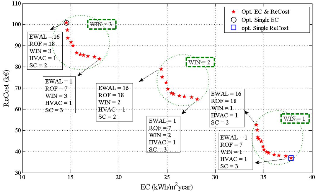
Figure 6 Multi-objective solutions for the building retrofit strategies (EC - ReCost) (Refer to Appendix A for RAs characteristics)
