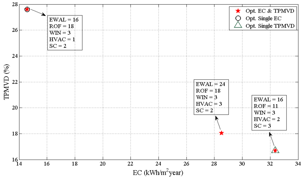
Figure 5 Multi-objective solutions for the building retrofit strategies (EC – TPMVD) (Refer to Appendix A for RAs characteristics)
