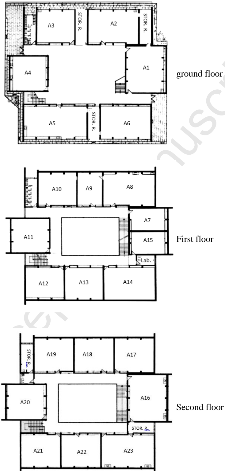
Figure 4 Schematic plan of ground, first and second floor of the case study
