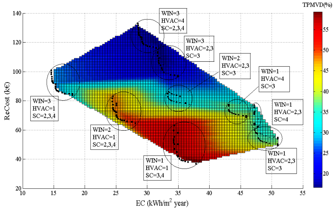
Figure 9 Results of multi-objective optimization of EC, ReCost and TPMVD - 2D projection (EC – ReCost) (Refer to Appendix A for RAs characteristics)
