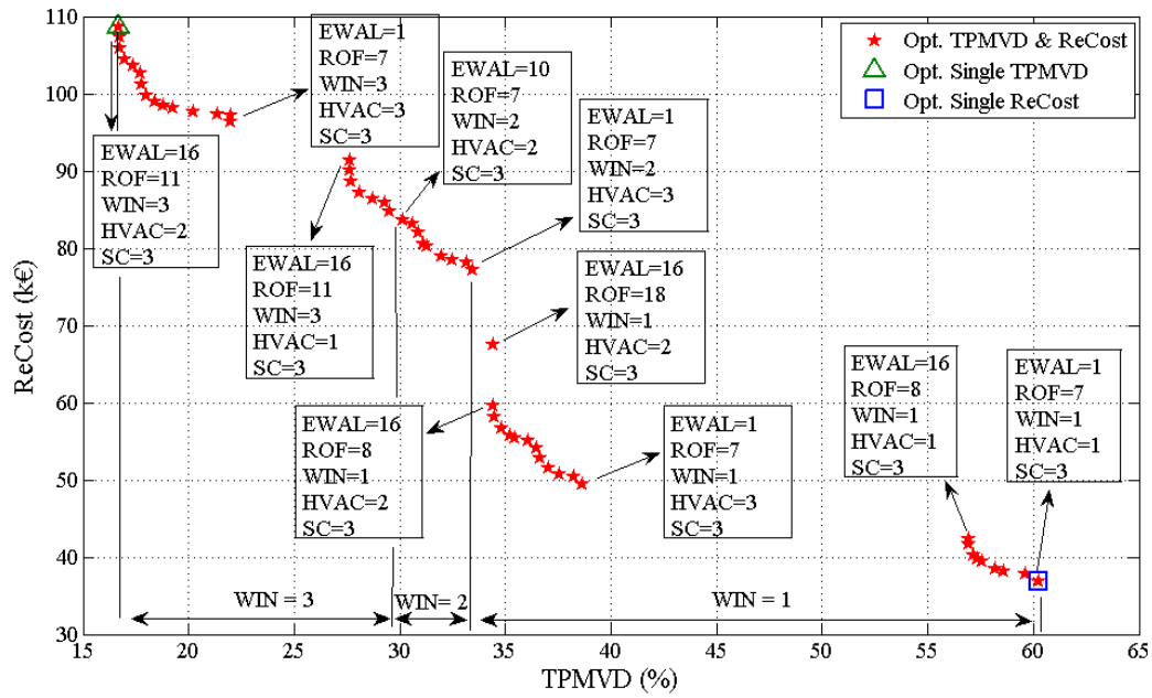
Figure 7 Multi-objective solutions for the building retrofit strategies (TPMVD - ReCost) (Refer to Appendix A for RAs characteristics)
