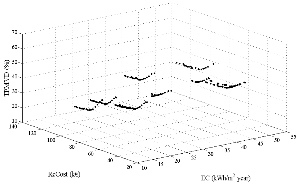
Figure 814 Results of multi-objective optimization - 3D visualization
