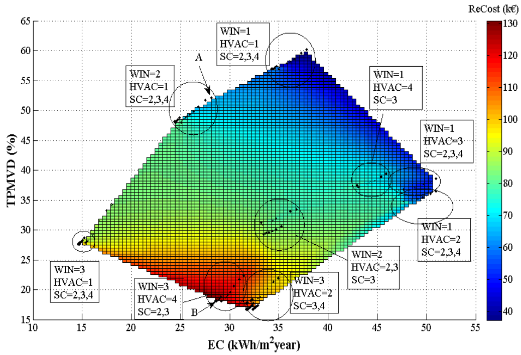
Figure 10 Results of multi-objective optimization of EC, ReCost and TPMVD - 2D projection (EC – TPMVD) (Refer to Appendix A for RAs characteristics)
